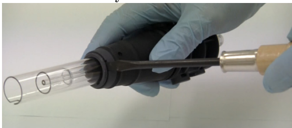
Figure 9. Separating the torch securing ring from the torch body
