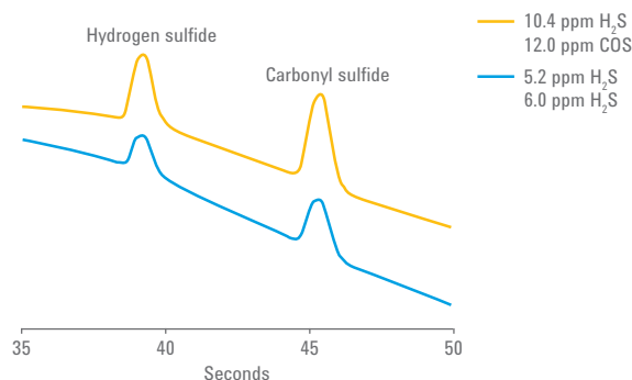
Micro-machined thermal conductivity detector
