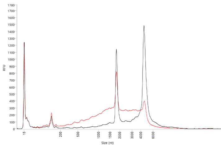
Figure 1. Universal mouse reference total RNA separated on the Agilent Fragment Analyzer system with the HS RNA kit (p/n DNF-472). Sample at 0 (black) and 8 (red) minutes at 70°C. RQN = 9.6 & 6.2, respectively.
