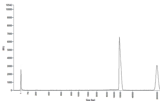
Figure 4. 15,000 bp DNA fragment separated using the HS Large Fragment 50 kb kit (p/n DNF-464) on the 5200 Fragment Analyzer system. Large DNA fragments of all origins can be separated on these systems.
