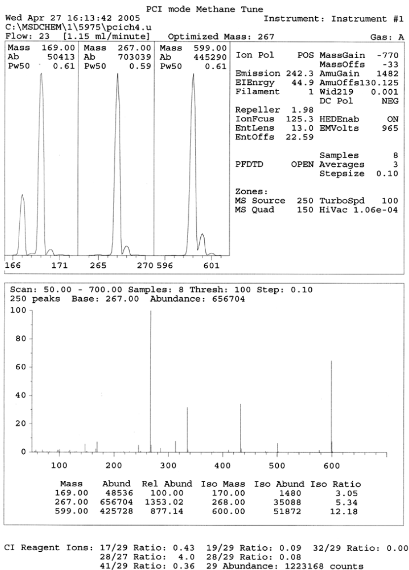
Figure 30 PCI autotune
