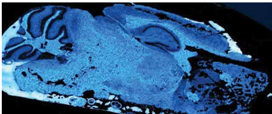
Figure 4. A chemical image of a mouse brain slice showing lipid distribution (12mm x 7mm) at 1 \mu\text{m} pixel measured in 1 hour.
