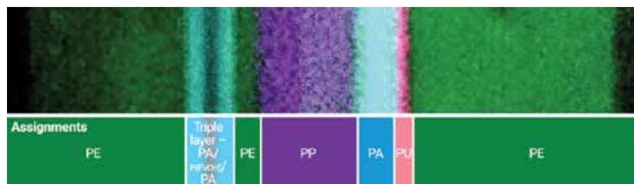
Figure 5. A chemical image showing layers of the laminate sample (120 \mu\text{m} width) consisting of polyethylene (PE), polyamide (PA), poly (ethylene vinyl alcohol) (P(EVOH)), polypropylene (PP) and polyurethane (PU). The thinnest layer observed was only 2.6 \mu\text{m} thick.
