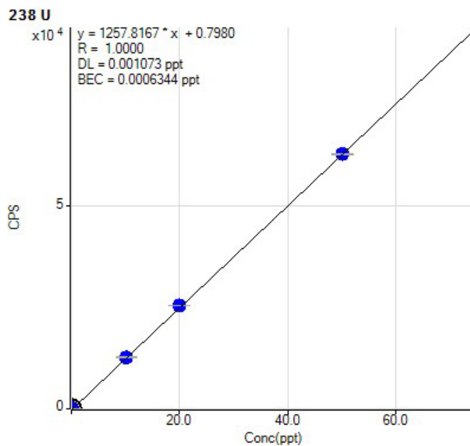
Figure 3. Calibration curve of 232 Th (left) and 238 U (right). The DLs of 2 ppq (Th) and 1 ppq (U) were calculated as three times the standard deviation of 10 replicate analyses of the calibration blank with a 3 s integration time.
