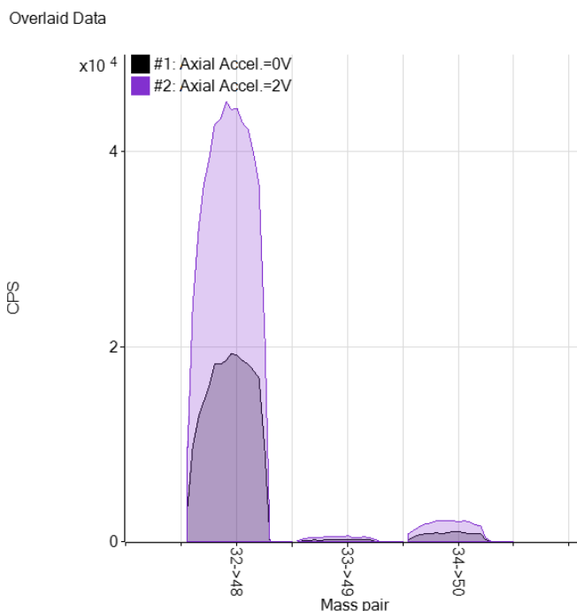
Figure 5. Spectrum of 50 ppb sulfur with and without axial acceleration, showing significant signal enhancement with axial acceleration voltage.
