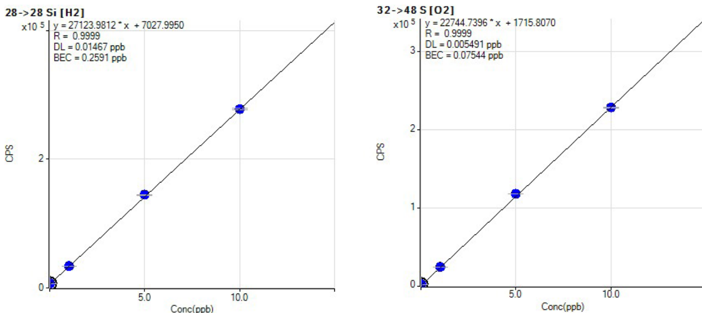
Figure 4. Left: calibration curve of silicon in MS/MS on-mass mode using H 2 cell gas; a DL of 15 ppt was achieved. Right :calibration curve of sulfur in MS/MS mass-shift mode using O 2 cell gas; a DL of 5 ppt was achieved.
