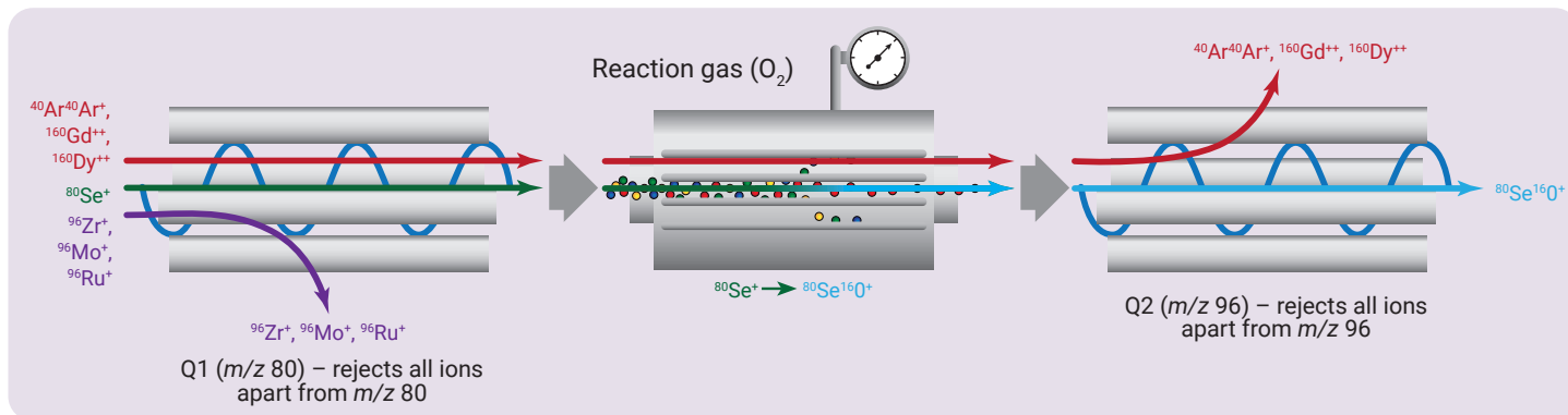
Figure 1B. ICP-QQQ with double mass selection (MS/MS). Q1 allows only ions at m/z 80 to pass to the cell—all other ions are rejected. ^{80}\text{Se}^+ is converted to ^{80}\text{Se}^{16}\text{O}^+ in the cell with \text{O}_2 reaction gas. Q2 measures \text{SeO}^+ at m/z 96. Zr, Mo, and Ru cannot interfere at m/z 96, since they were rejected by Q1.
