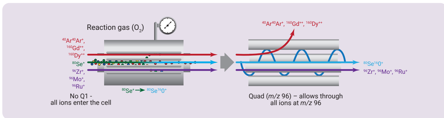
Figure 1A: Conventional single quadrupole or bandpass ICP-MS. Using \text{O}_2 reaction gas, Se is reacted away from interferences ( \text{Ar}_2^+ , \text{Gd}^{++} and \text{Dy}^{++} ) at m/z 80. ^{80}\text{Se}^+ is converted to ^{80}\text{Se}^{16}\text{O}^+ in the cell and measured at m/z 96. However, Zr, Mo, and Ru also contribute ions at m/z 96, leading to incorrect Se data.
