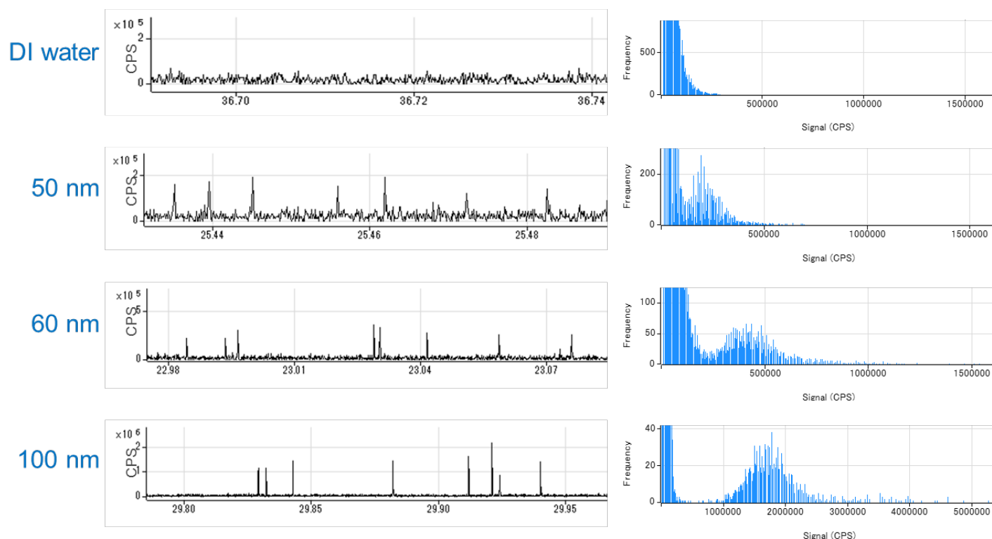
Figure 6. Left: single particle analysis of blank and SiO 2 NP standards in fast TRA mode. Right: size frequency distribution plots calculated for SiO 2 NPs from the TRA data.
