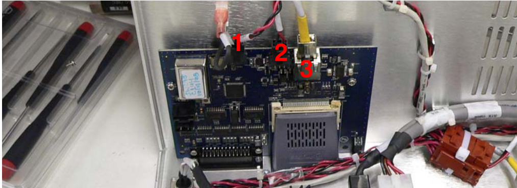
Figure B-39 Discrete I/O Board Wiring
