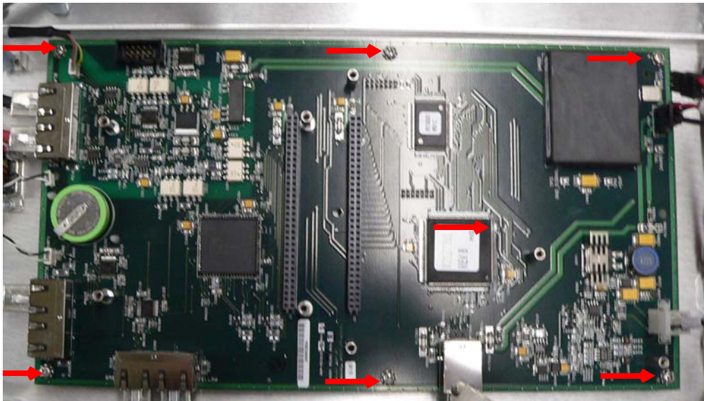
Figure B-37 Mother Board Mounting Screws
