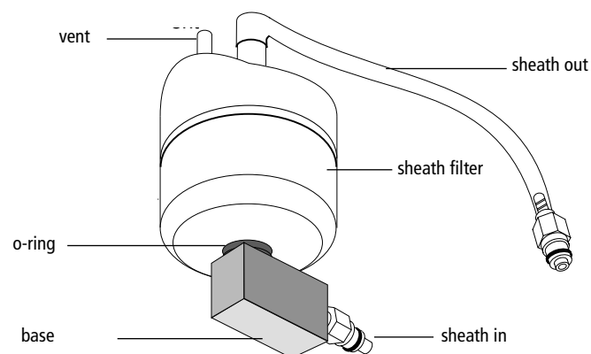
Figure 2-12 Sheath Filter
