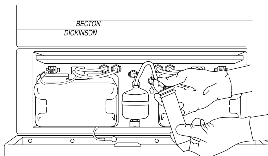
Figure 2-10 Venting Air from Sheath Filter
