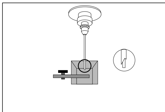
Figure 2-3 Sample Injection Port
