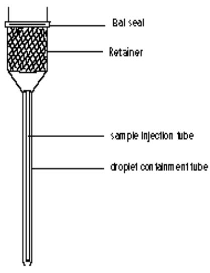
Figure 2-13 Bal Seal
