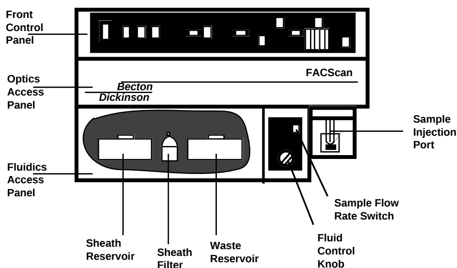
Figure 2-1 BD FACScan Sensor Module
