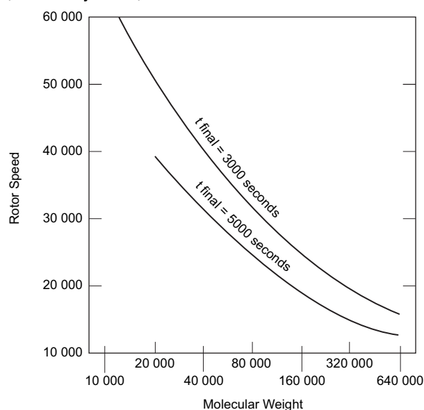
Figure 4.2 Plot of Suggested Rotor Speed Versus Molecular Weight for Two Data Collection Times (L. Holladay, 1980)
