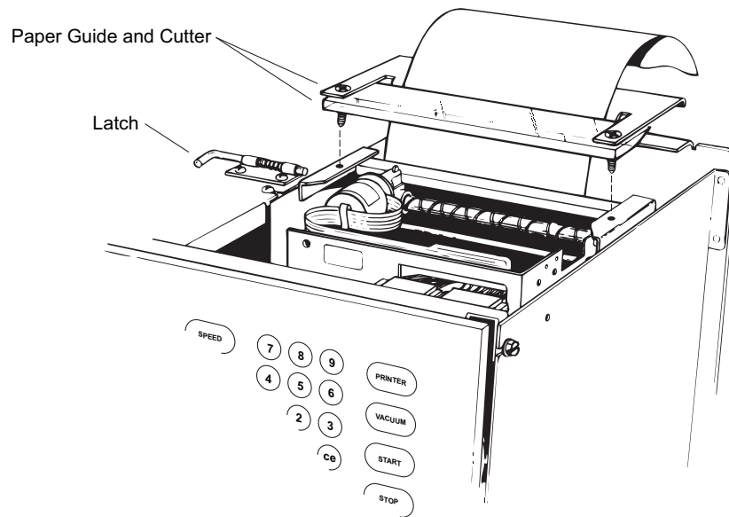
Figure 5.9 Removing the Paper Guide and Plastic Cutter
