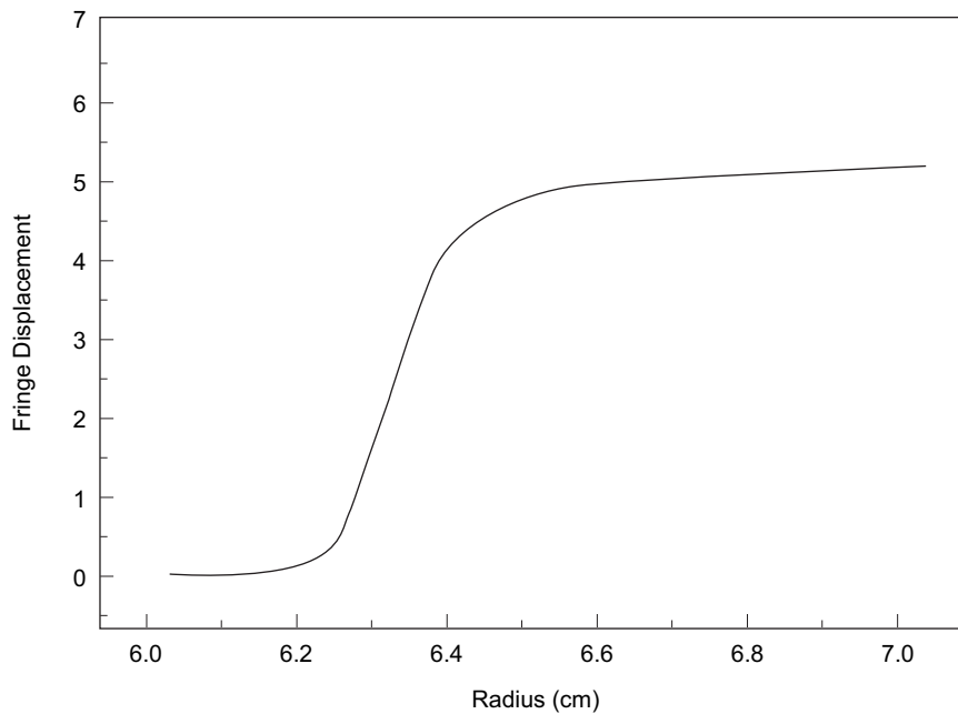
Figure 2.9 Plot of Interference Data Resulting from Fast Fourier Transformation
