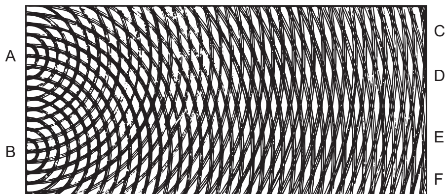
Figure B.2 Thomas Young's Original Drawing of a Two-Source Interference Pattern
