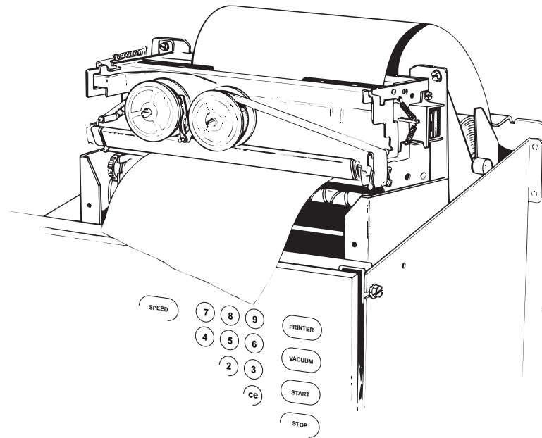
Figure 5.11 Ribbon Spools Installed
