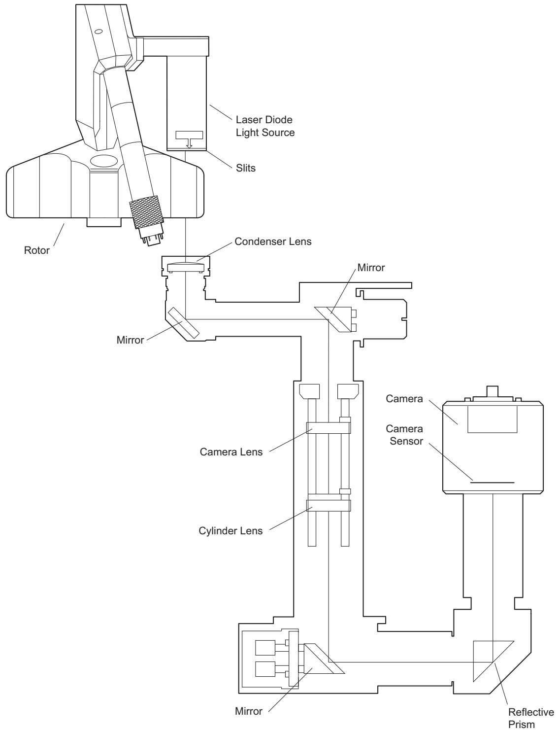
Figure 2.7 The XL-I Interference Optical System
