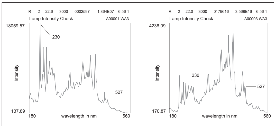
Figure 5.7 Wavelength Scans of a Windowless Cell in a Calibrated XL-A or XL-I
