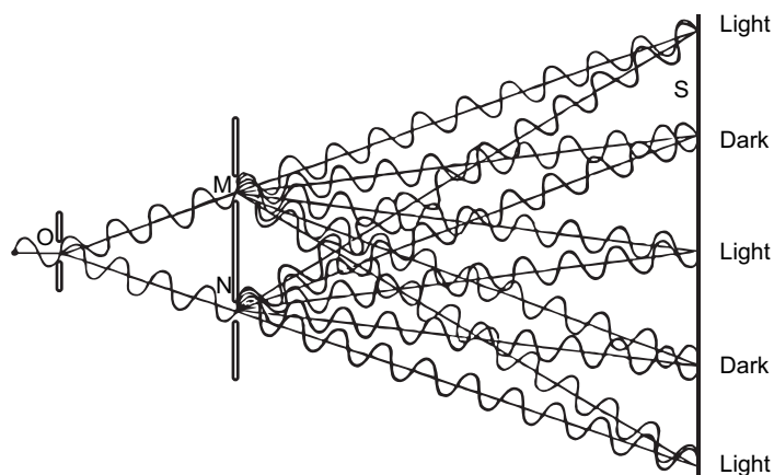
Figure B.4 Light from O passes Through Slits M and N and Produces an Interference Pattern on Screen S
