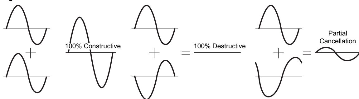
Figure B.1 Wave Interference
