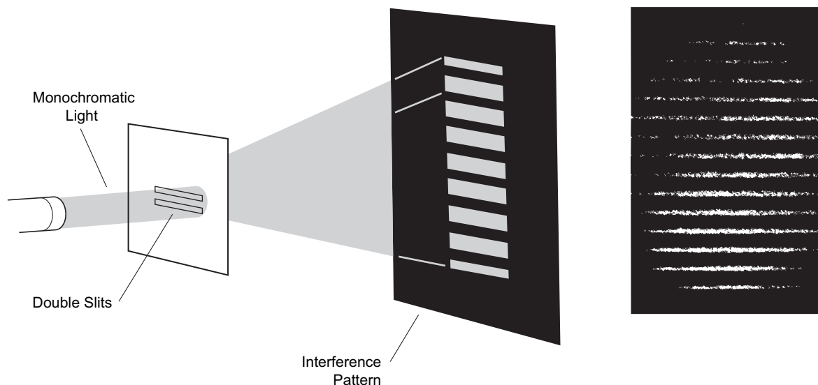
Figure B.3 Interference Pattern Created by Two Slits
