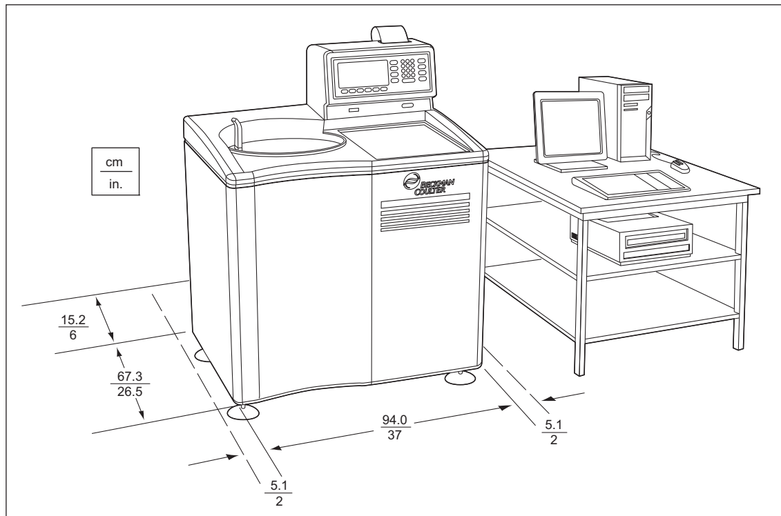
Figure A.2 ProteomeLab XL-A or XL-I Instrument and Data System Space Requirements
