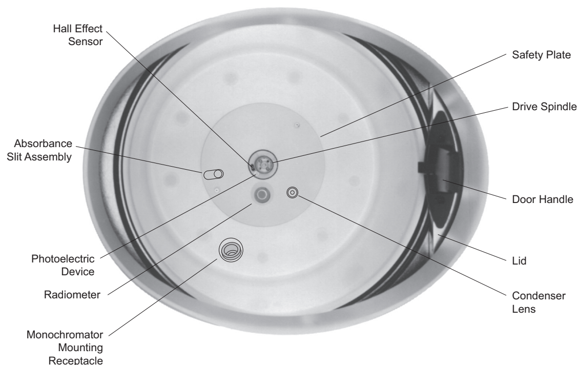
Figure 2.1 The Rotor Chamber
