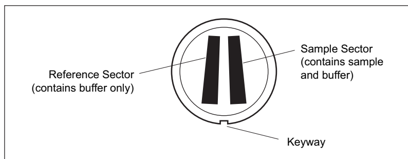
Figure 2.5 Top View of Reference and Sample Sectors in a Two-Channel Cell
