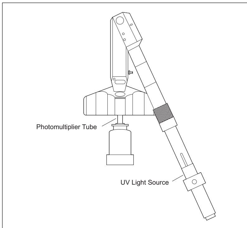
Figure 2.2 The XL-A Monochromator
