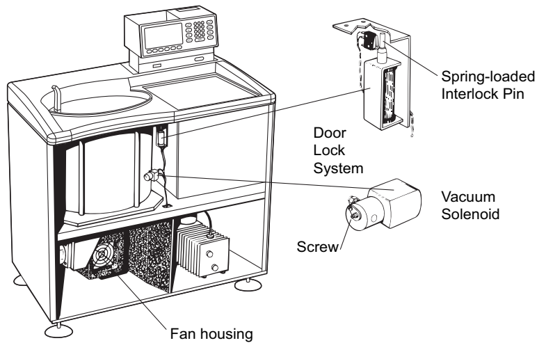
Figure 5.3 Interior View of Instrument (Panel Removed)
