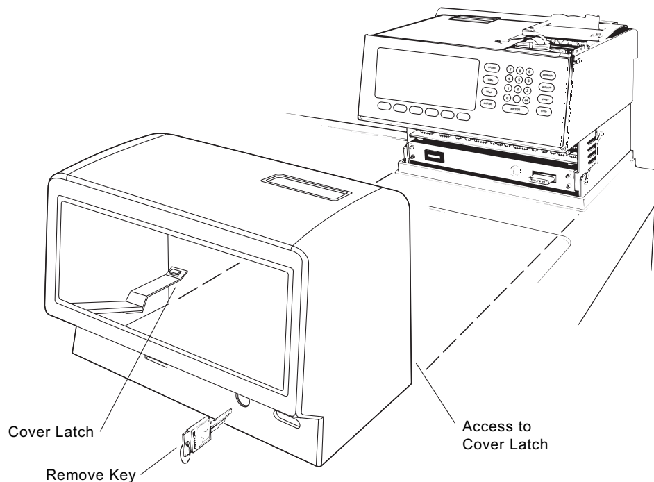
Figure 5.1 Removing the Control Head Cover
