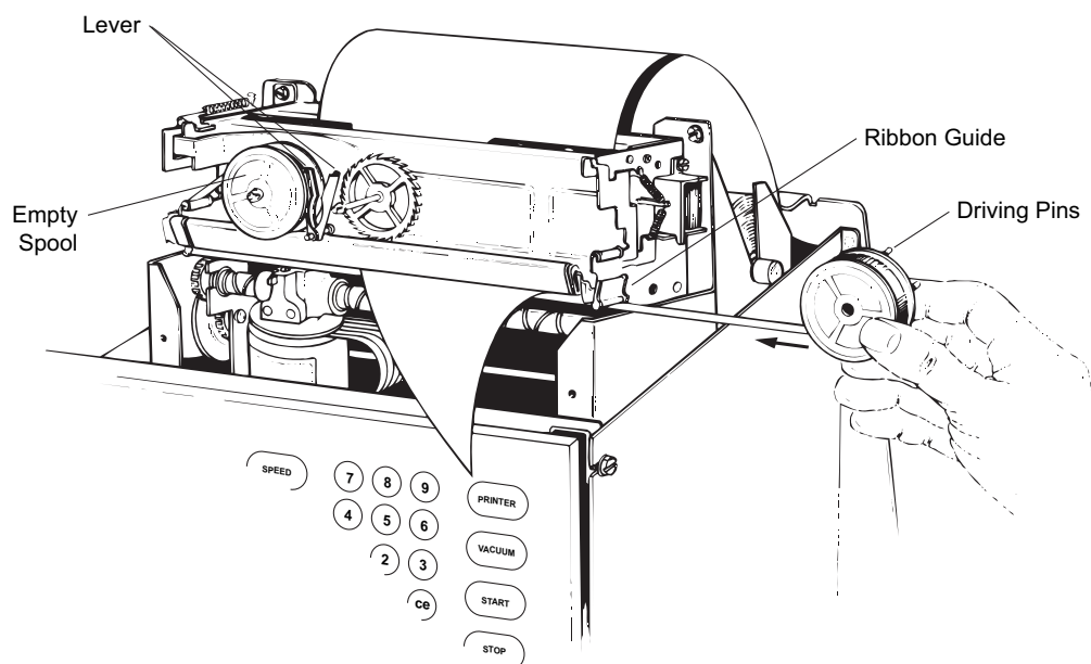
Figure 5.10 Inserting the New Ribbon
