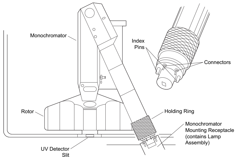
Figure 2.13 Installing the Monochromator (XL-I monochromator shown)
