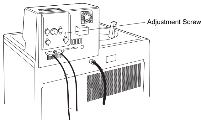
Figure 5.6 Location of the Screw that Adjusts Video Brightness
