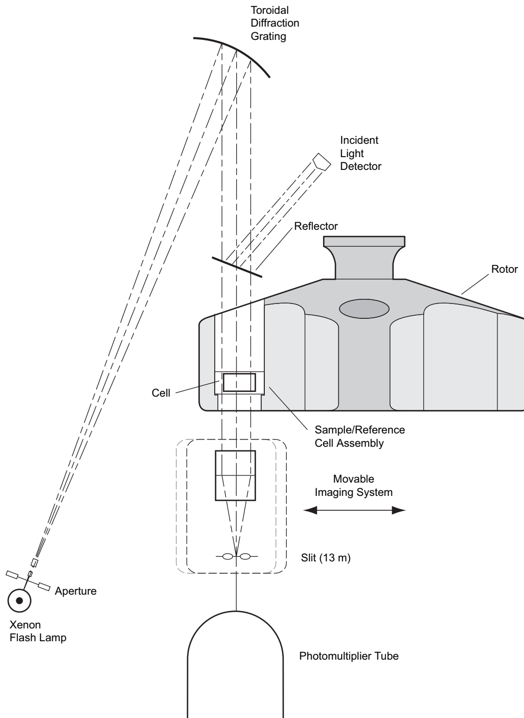
Figure 2.4 The Scanning UV/VIS Absorbance Optical System
