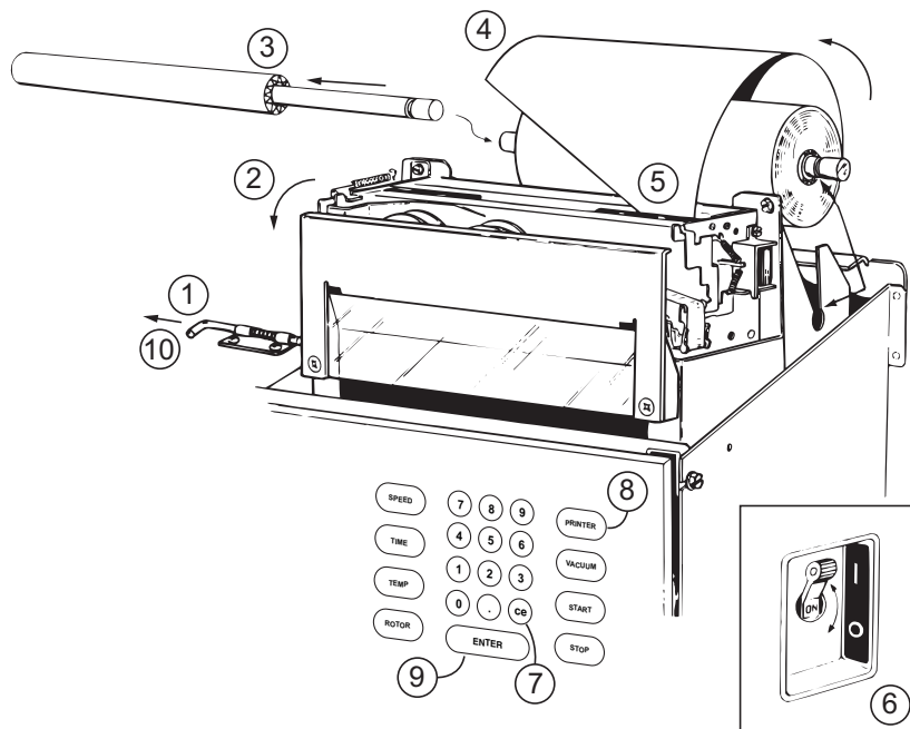
Figure 5.8 Printer Assembly in Raised Position
