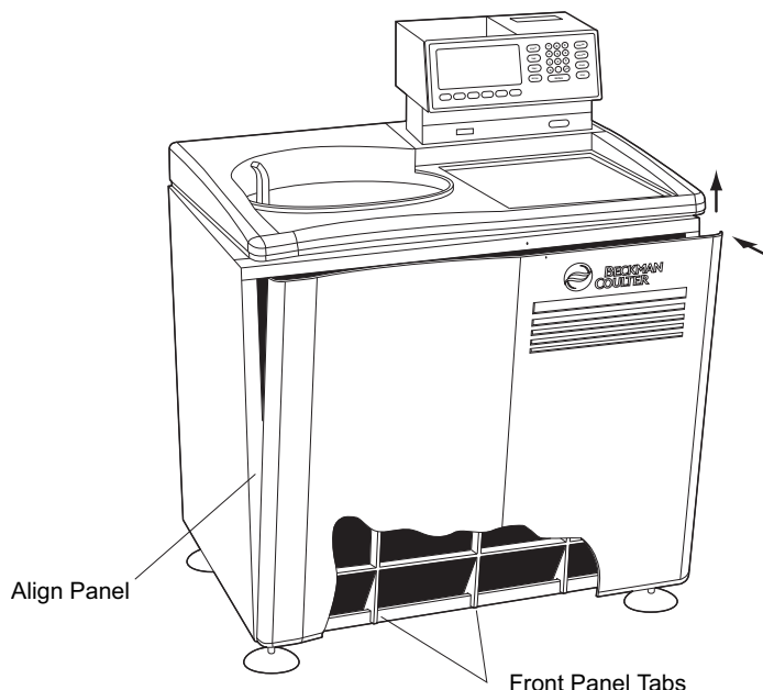
Figure 5.4 Reinstalling the Front Panel
