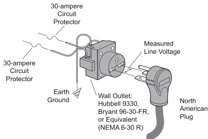
Figure A.1 ProteomeLab XL-A or XL-I Electrical Requirements
