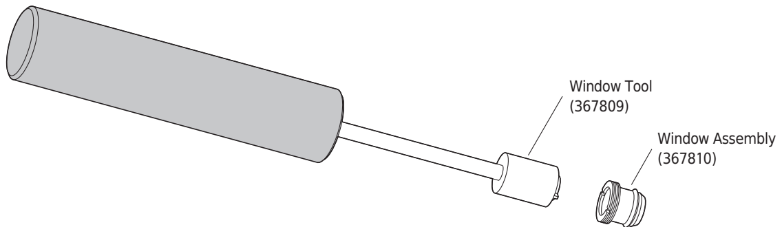
Figure 5.5 Monochromator Window Assembly and Window Installation and Removal Tool
