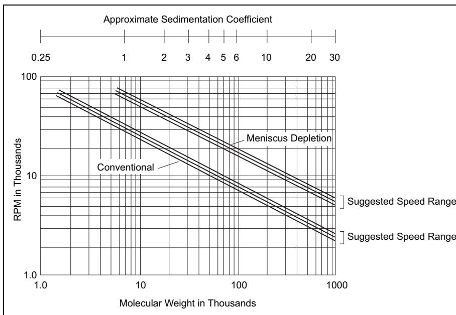
Figure 4.3 Rotor Speed Selection Chart for Sedimentation Equilibrium Runs
