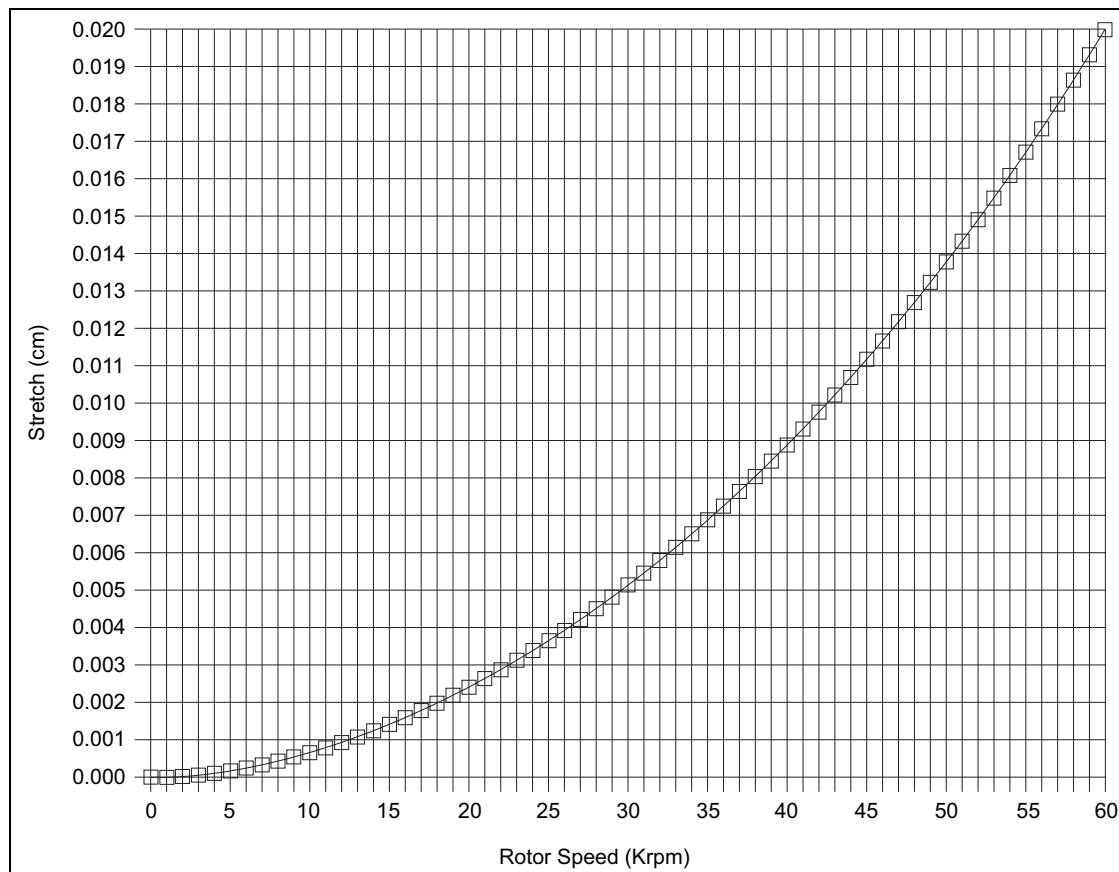
Figure 4.1 An-60 Ti Rotor Stretch at Outer Cell Wall
