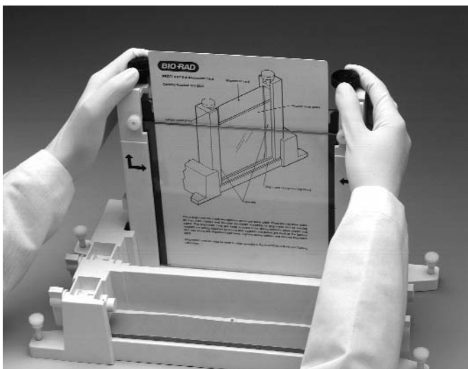
Fig. 5.4. Aligning spacers in the sandwich assembly.
