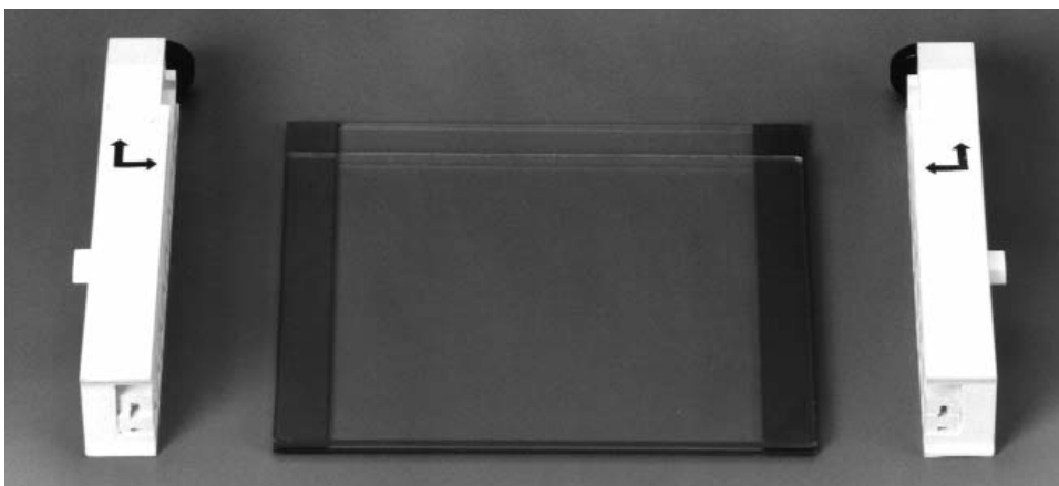
Fig. 6.3. Positioning glass plates, spacers, and clamps.
