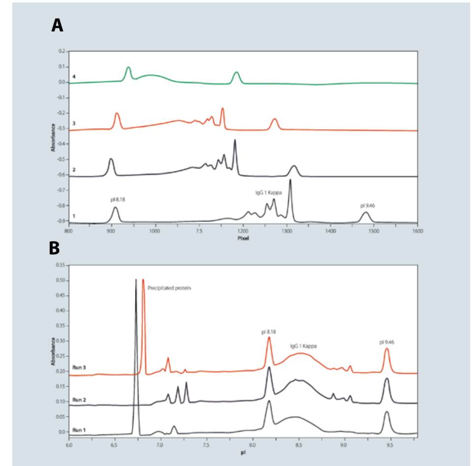
Figure 3. The separation of IgG 1 Kappa demonstrates the adverse effects of salts (A). Triplicate runs at 100 mM NaCl show that salt also affects reproducibility (B).
