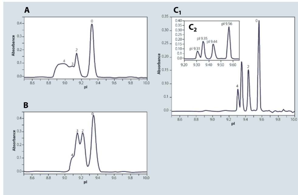
Figure 2. The complete icIEF method development process—from the screening of compounds in a pH gradient (A), to the addition of solubilizers (B), to the addition of narrow-range ampholytes (C)—can be completed in 2.5 hours.
