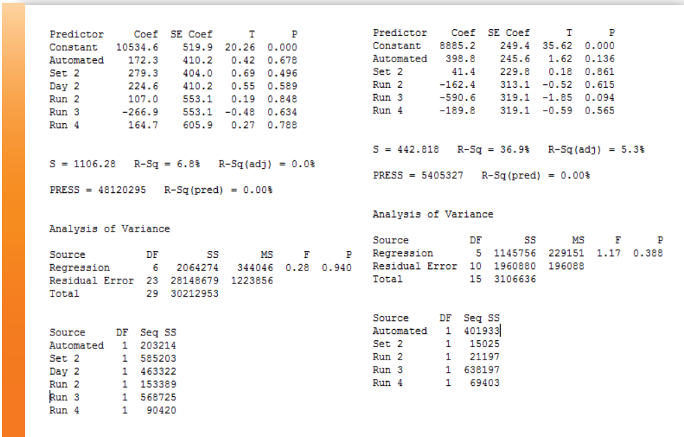
Figure 3. Linear regression analysis was used with dummy coding to evaluate relevant variables (manual method, automated method, day) as a group. Analysis shows no significant impact of system inputs (automation, day to day variance) on particle counts. The various system inputs could account for 0.0% (ProteinSimple, left) and 5.3% (Takeda, right) of the variation in the data. An R-Sq (adj) of >30% would indicate a significant impact.
