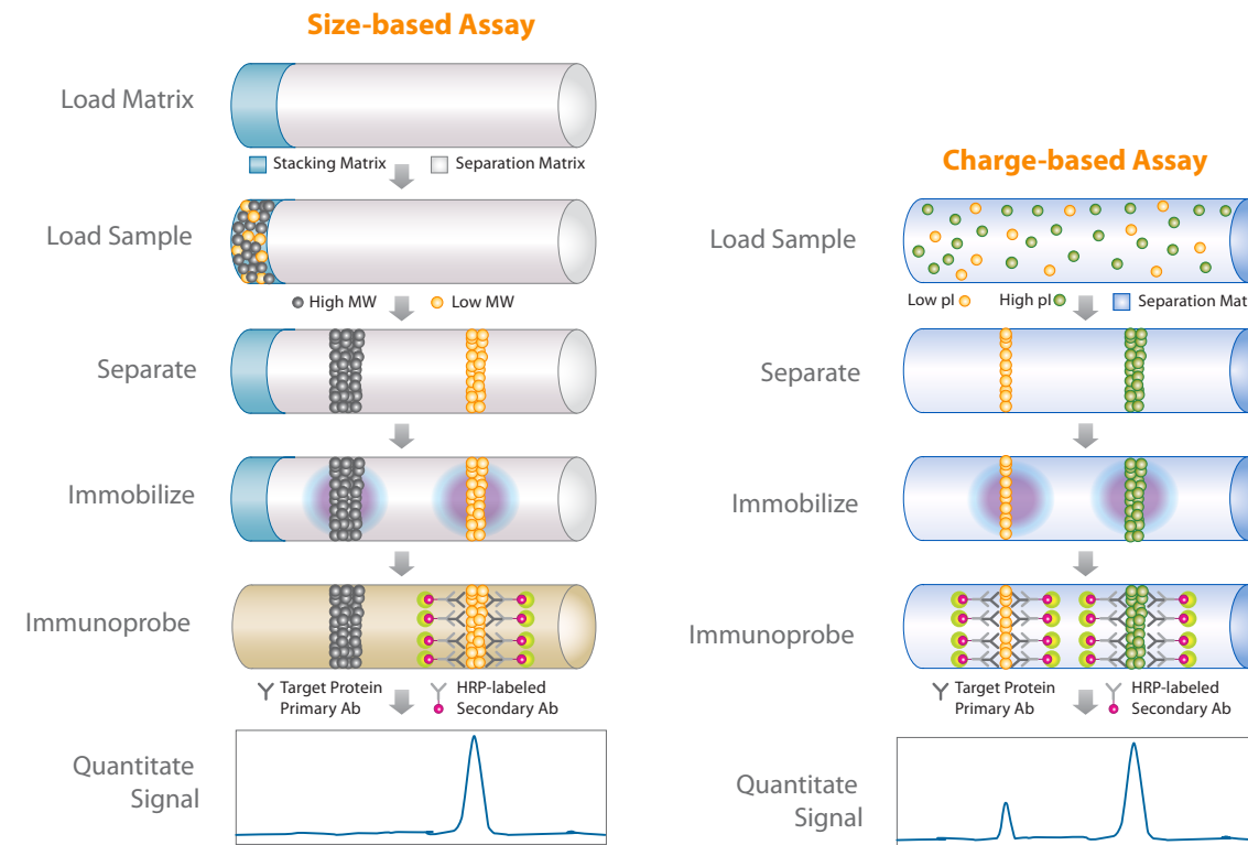
Figure 1. Simple Western assays combine a familiar separation technique, capillary electrophoresis, with a well-known detection technique, an immunoassay, to give you quantifiable, highly reproducible data.
