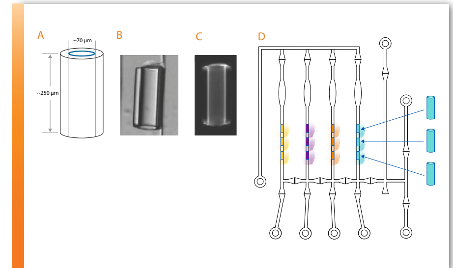
Figure 1. The Glass Nano Reactor (GNR). (A) Physical dimensions of a GNR. (B) Photograph of a GNR embedded in the channel of the Simple Plex cartridge. (C) Fluorescent image of a GNR revealing exclusive localization of antibodies in the center of the GNR, with no detectable signal on the outer surfaces. (D) Cartoon depicting placement of GNRs in discrete channels of one of the eight circuits on an 8-sample 4-plex cartridge. Different colors indicate GNRs specific for different analytes.
