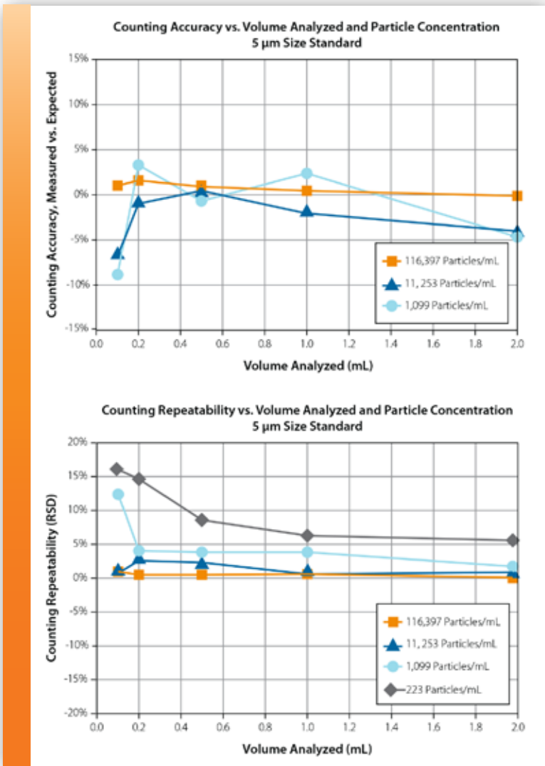
Figure 2. Impact of volume on counting accuracy for differing particle concentrations (top). Impact of volume on counting reproducibility for differing particle concentrations (bottom).
