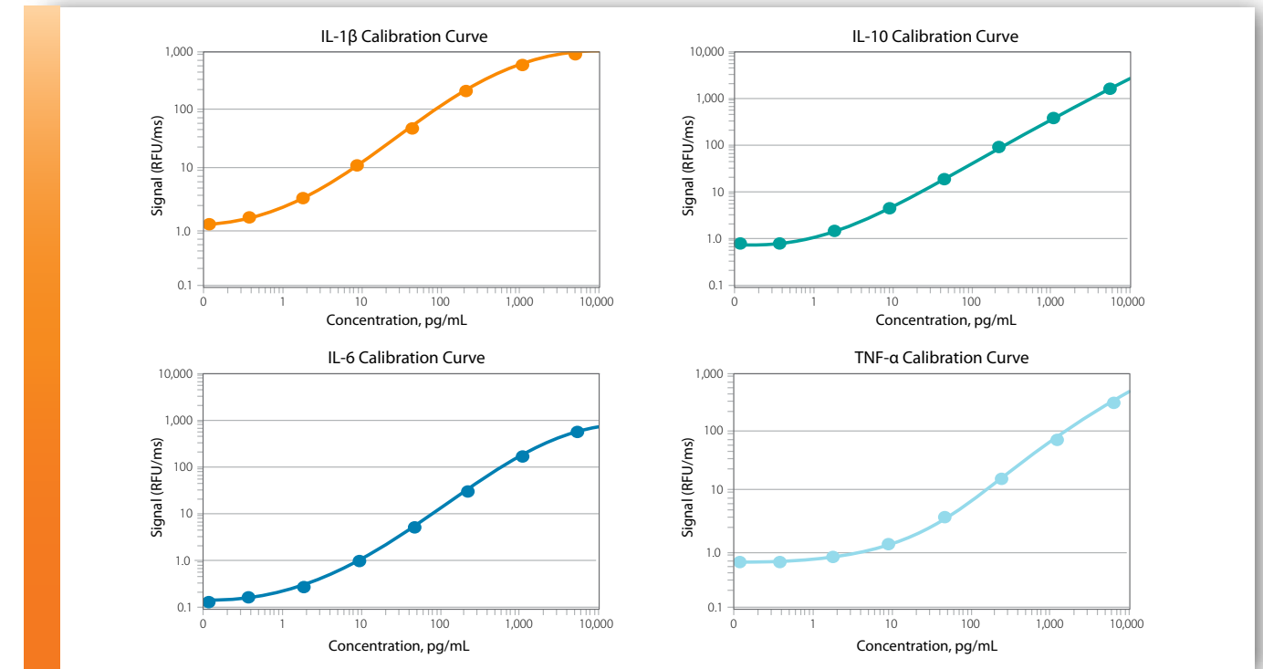
Figure 3. Calibration curves for the individual biomarkers run in the Simple Plex assay format. Data points are the average of a minimum of four data points per day over five days with standard deviation error bars.
