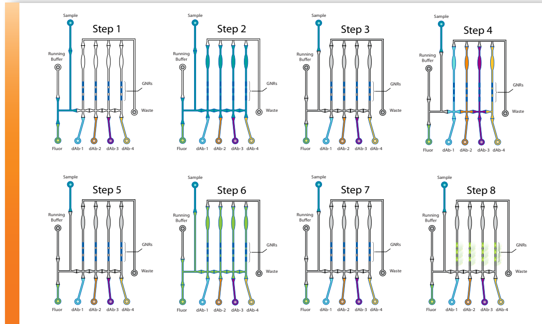
Figure 2. The Simple Plex assay work flow, shown for one of the eight sample circuits. Step 1: The system is primed with sample. Step 2: Sample is pumped through the circuit and split evenly between the four channels containing analyte-specific GNRs. Step 3: After sample incubation, the circuit is cleaned with wash buffer. Step 4: Analyte-specific dAb's are individually pumped into their respective channels to bind analyte captured on the GNRs. Step 5: Unbound dAb's are removed with wash buffer. Step 6: Detect fluor is flowed into all channels, binding bound dAb's. Step 7: Residual detect fluor is removed with wash buffer. Step 8: Detect fluors are excited with a 631 nm laser and the signal is read with a CCD camera.
