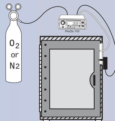
From outside the host chamber, the ProOx 110 works by remotely sensing oxygen inside the chamber and infusing gas to control to setpoint.
