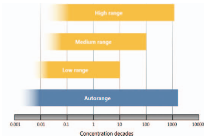
Figure 2 Automatic dynamic range selection selects the optimal reading range based on signal intensity in the well.
