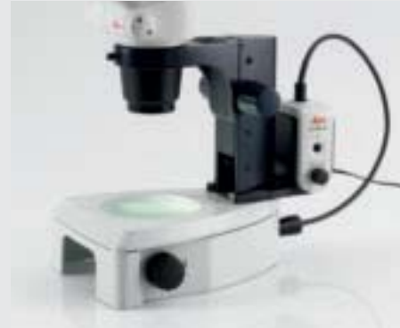
Sub-base for transmitted light and universal light guide for oblique transmitted illumination
