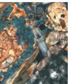
replacement aegirinitic grains. Crossed polarizers,
