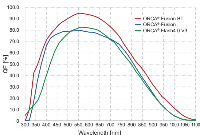
Figure 14. Quantum Efficiency of ORCA®-Fusion and ORCA®-Fusion BT.
