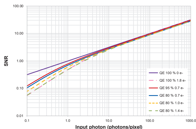
Figure 6. SNR curves show impact of read noise at low light.
