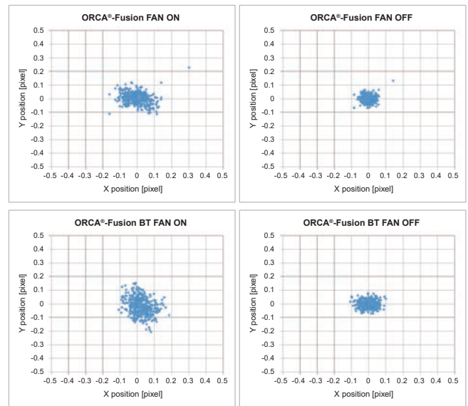
Figure 16. Fan vibration of ORCA®-Fusion / ORCA®-Fusion BT.
