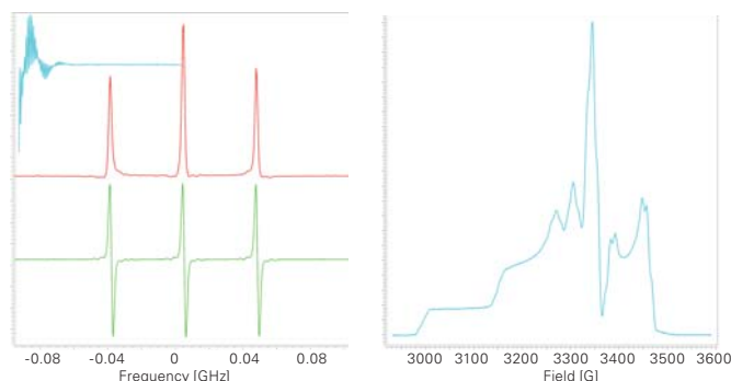
FT-EPR (red) spectrum 400 000 averages in 10 s. CW-EPR (green) spectrum 1 scan in 10 s.
