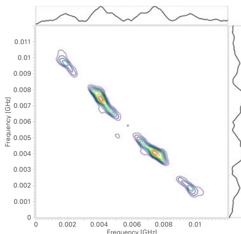
S-Band ^1\text{H} –HYSCORE of BDPA
