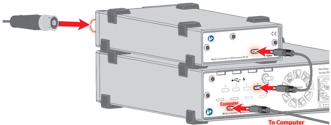
Figure 6-4 Connecting an instrument to the system using a PowerLab C
