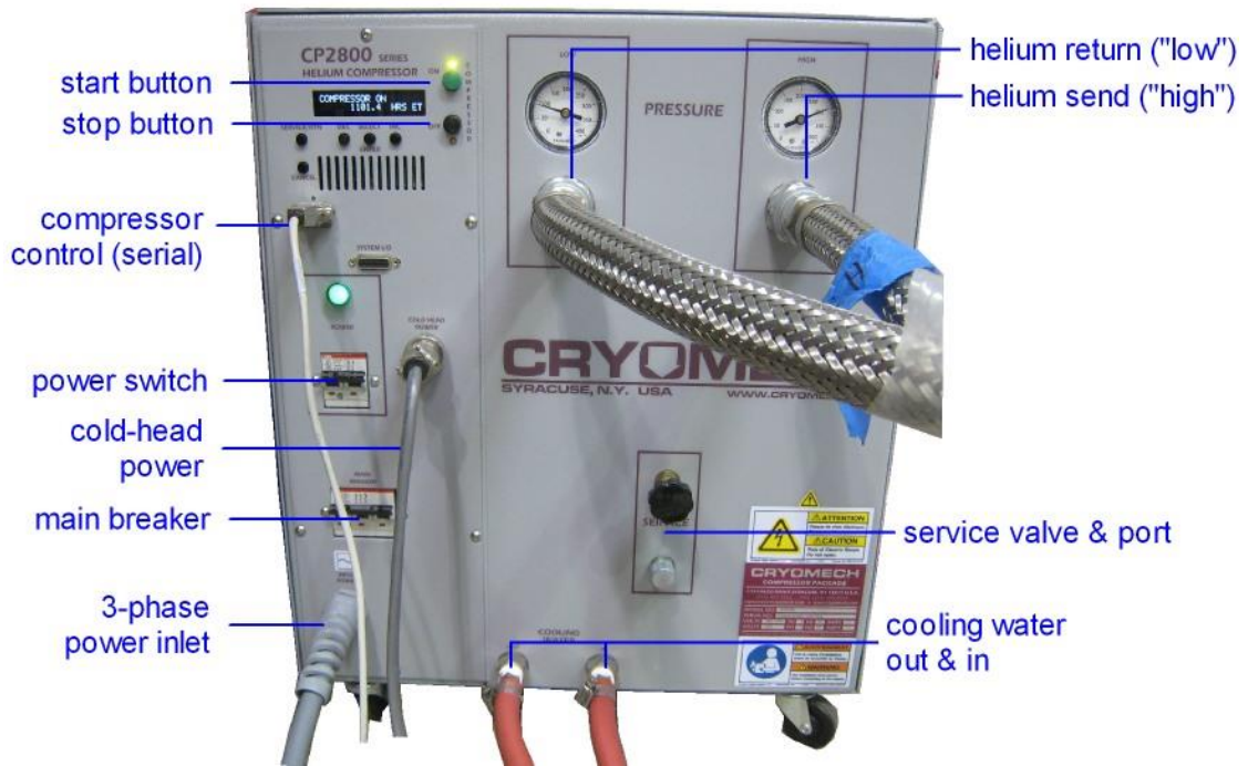
Figure 2-8. Helium Compressor.
