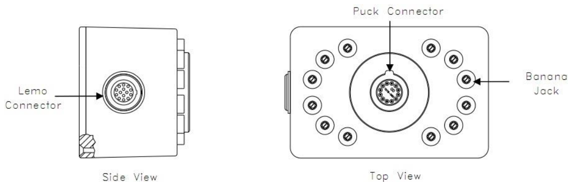
Figure 2-14. Puck Wiring Test Station
