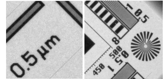
Left: True spatial resolution of 0.5 μm demonstrated on JIMA resolution target Right: True spatial resolution of 0.5 μm demonstrated on ZEISS Xradia resolution target
