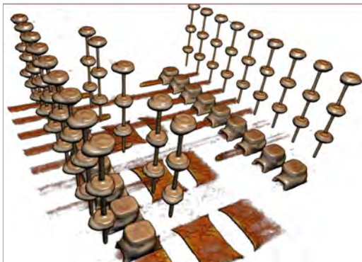
DRAM package interconnect within a 10 mm × 7 mm × 1 mm package containing a 4-die stack. Solder extrusion is easily visualized in 3 dimensions, 0.8 μm/voxel.
