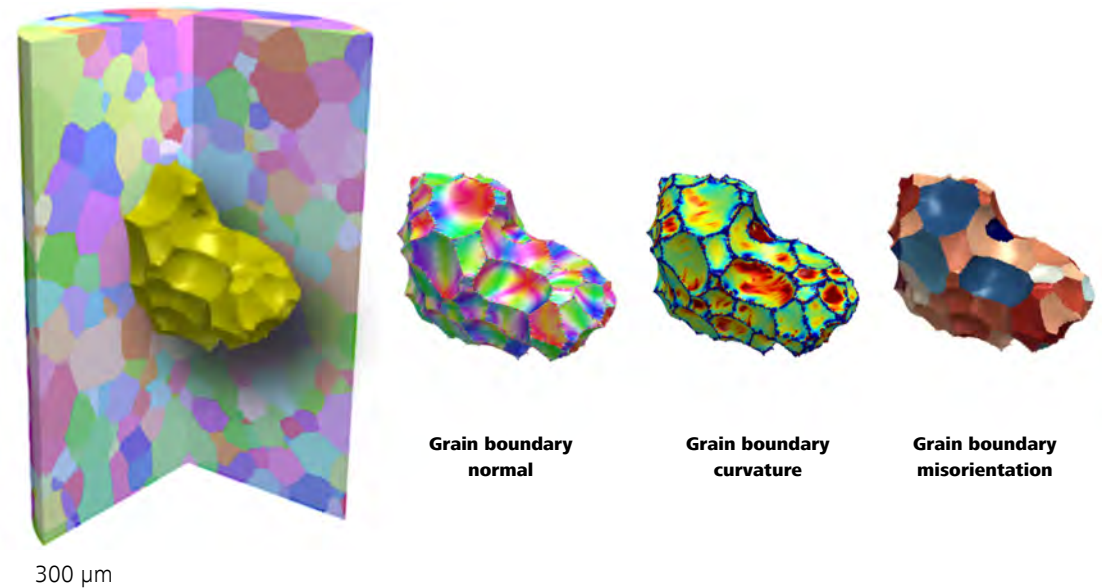
Armco iron sample with abnormal grain growth. Sample courtesy of Prof. Burton R. Patterson, University of Florida
