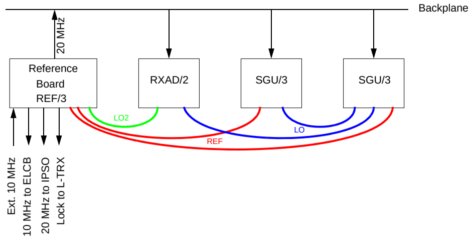
Figure 5.6 RF Distribution
