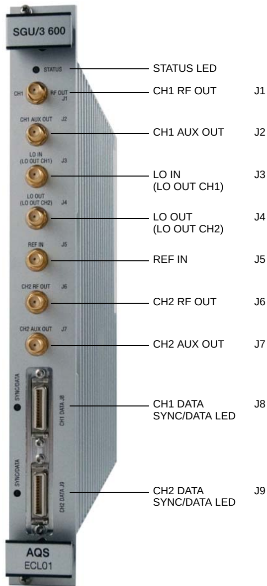
Figure 13.7 SGU/3 front panel
