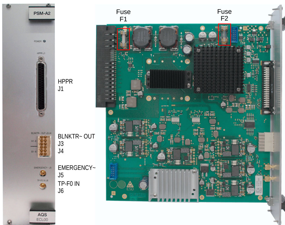
Figure 9.3 Overview PSM-A2
