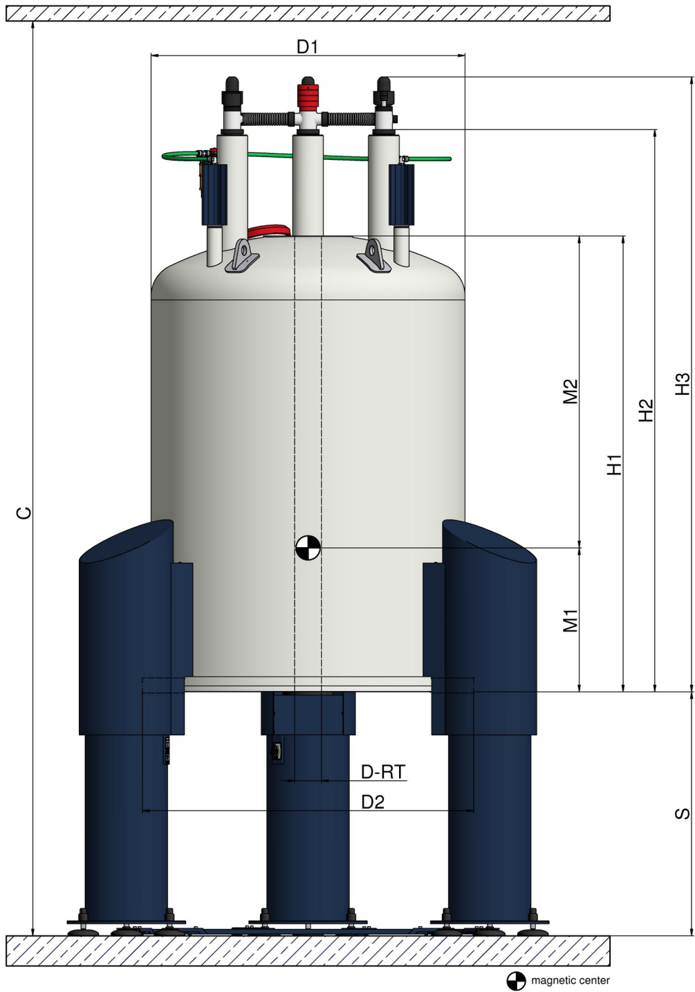
Figure 9.1: Dimensions of the Cryostat (front view)
