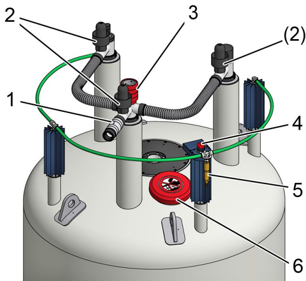
Figure 2.1: Safety Devices of the Cryostat with 3 Helium Turrets
