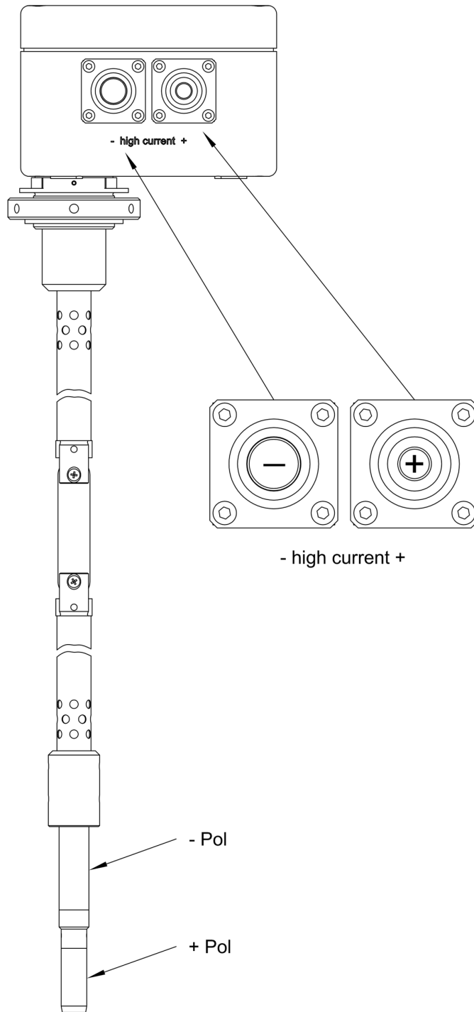
Figure 9.11: High Current Lead 2 Pin
