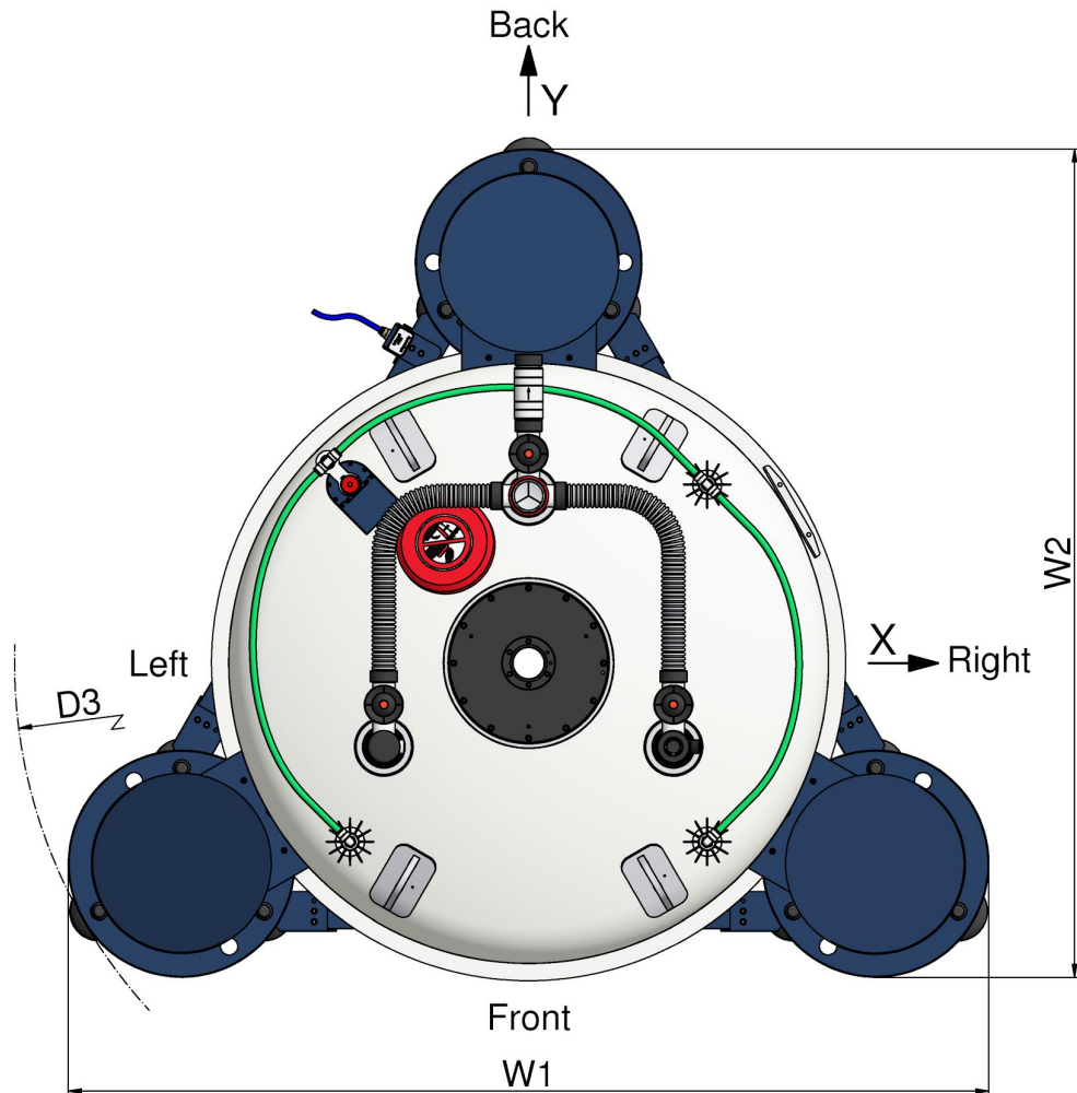
Figure 9.2: Dimensions of the Cryostat (top view)
