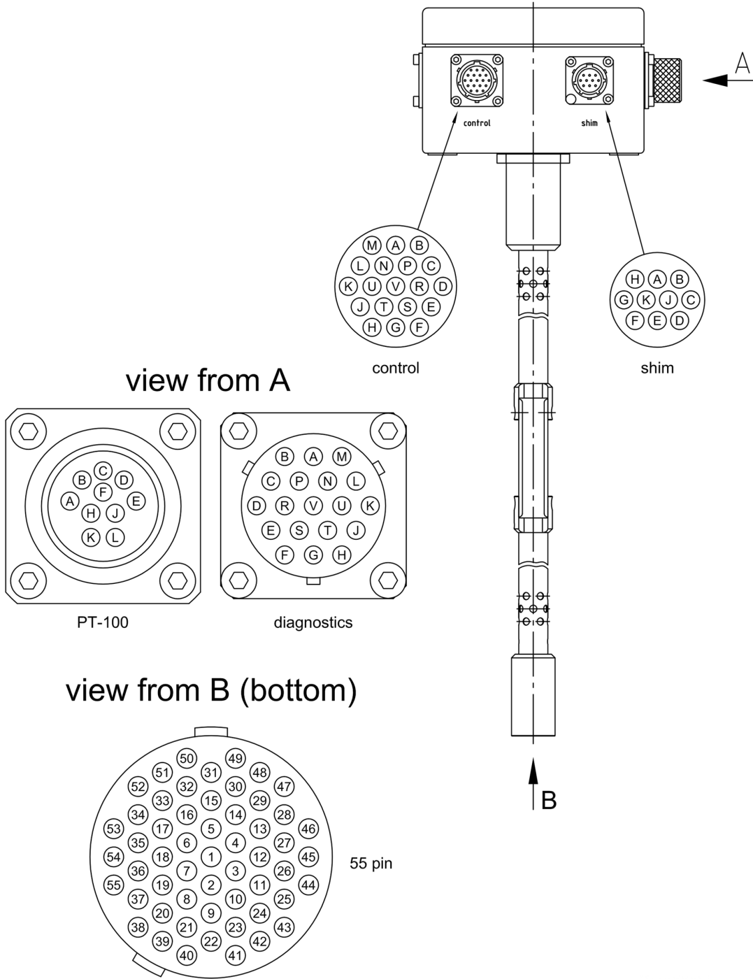
Figure 9.12: Diagnostic Lead 55 Pins
