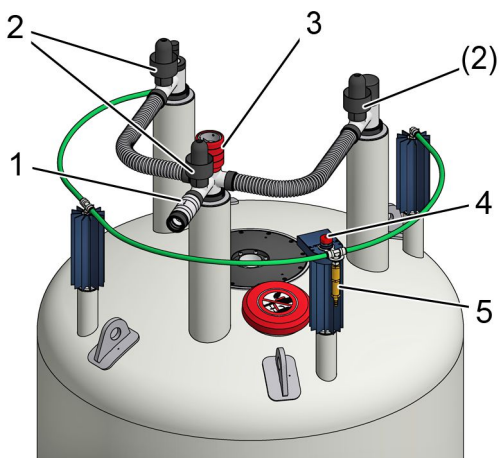
Figure 9.3: Safety Devices of the Cryostat with 3 Helium Turrets
