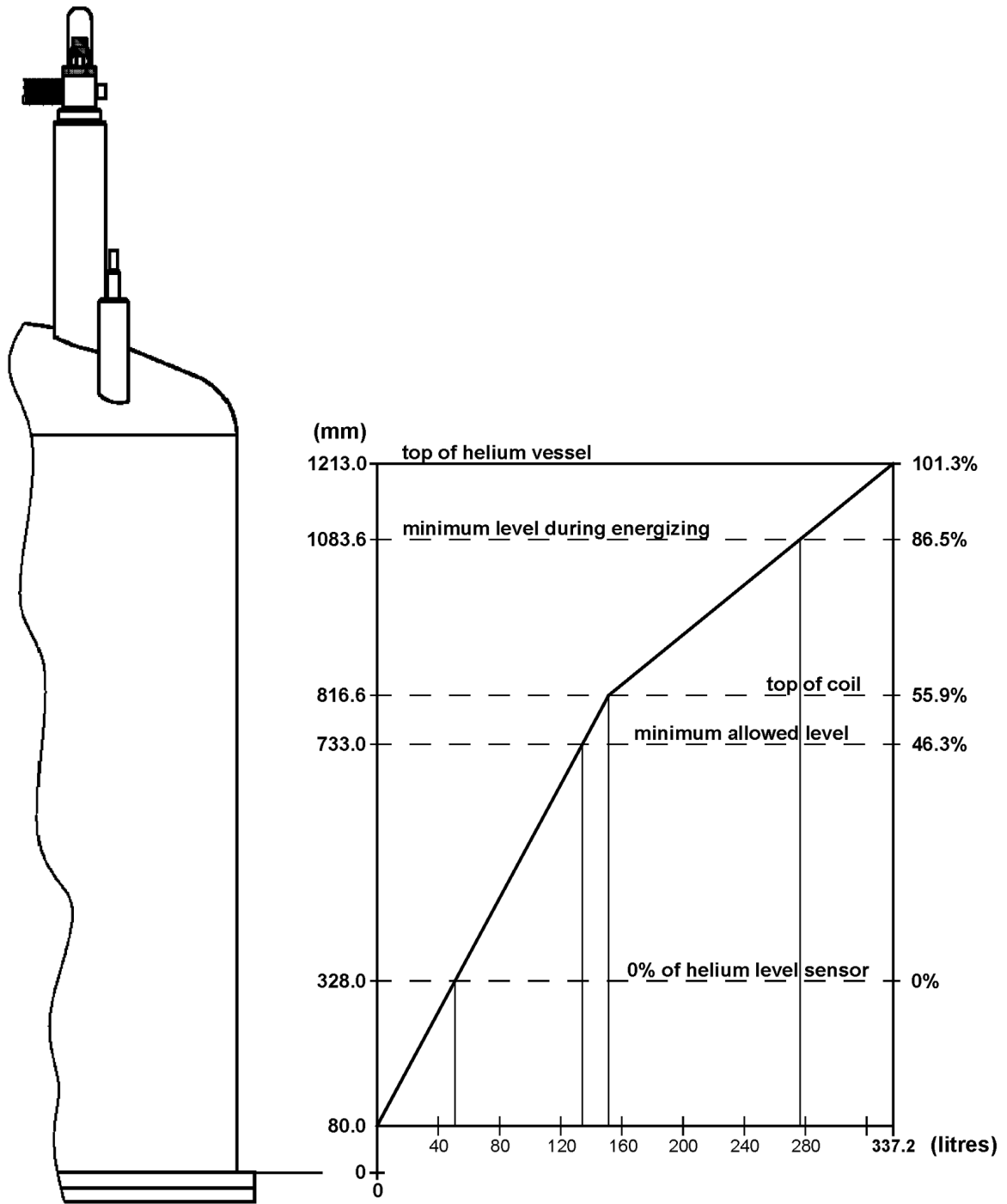
Figure 9.9: Helium Level Graph (800'54 Design D)
