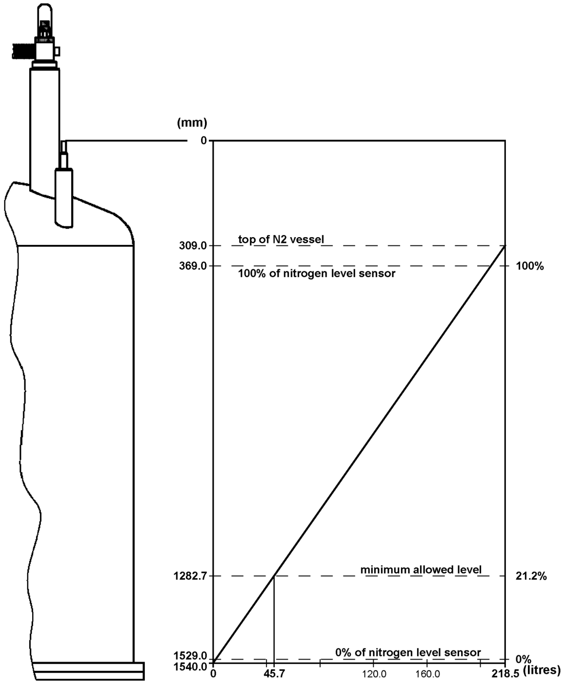
Figure 9.8: Nitrogen Level Graph (800'54 Design D)
