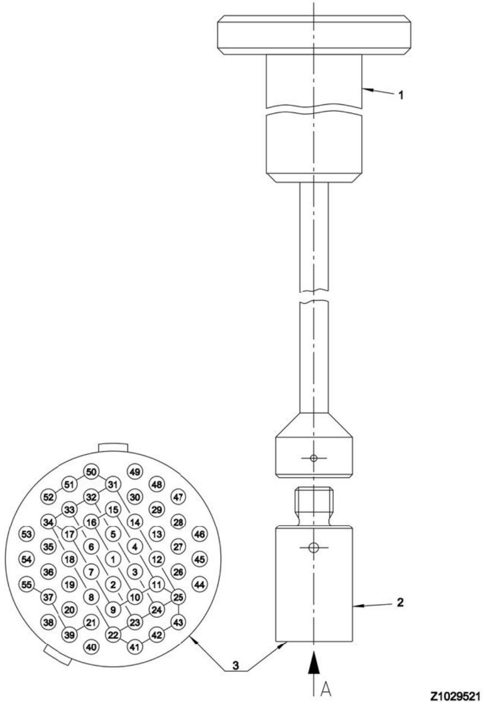
Figure 9.16: Shorting Plug 55 Pins
