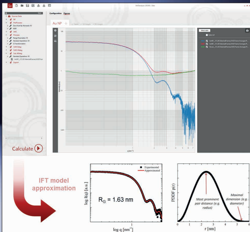
Size determination of dispersed gold nanoparticles
