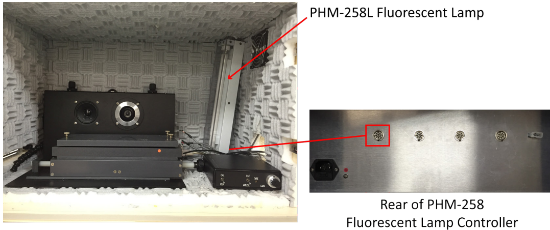
Figure 3-9 - Connect PHM-258L Lamp to PHM-258 Lamp Controller
