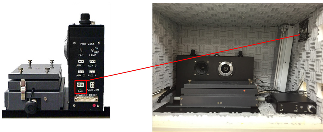
Figure 3-12 - Connect Fan to PHM-255A
