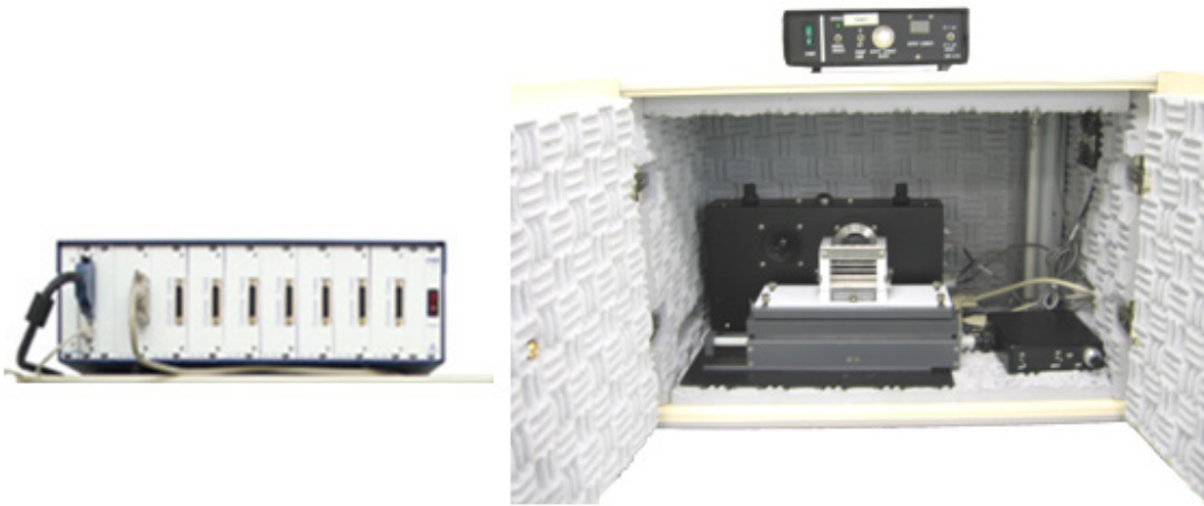
Figure 2-7 - Startle Reflex System Assembled
