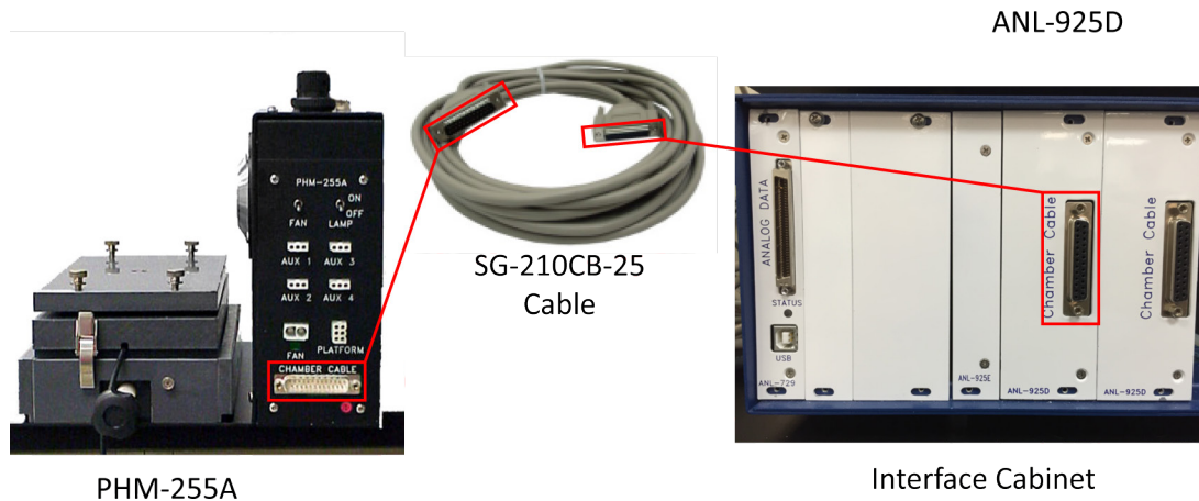
Figure 3-5 - PHM-255A Startle Platform to ANL-925D Card
