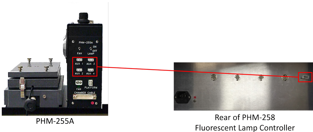
Figure 3-10 - Connect PHM-258 Lamp Controller to PHM-255A Stimulus Control Panel
