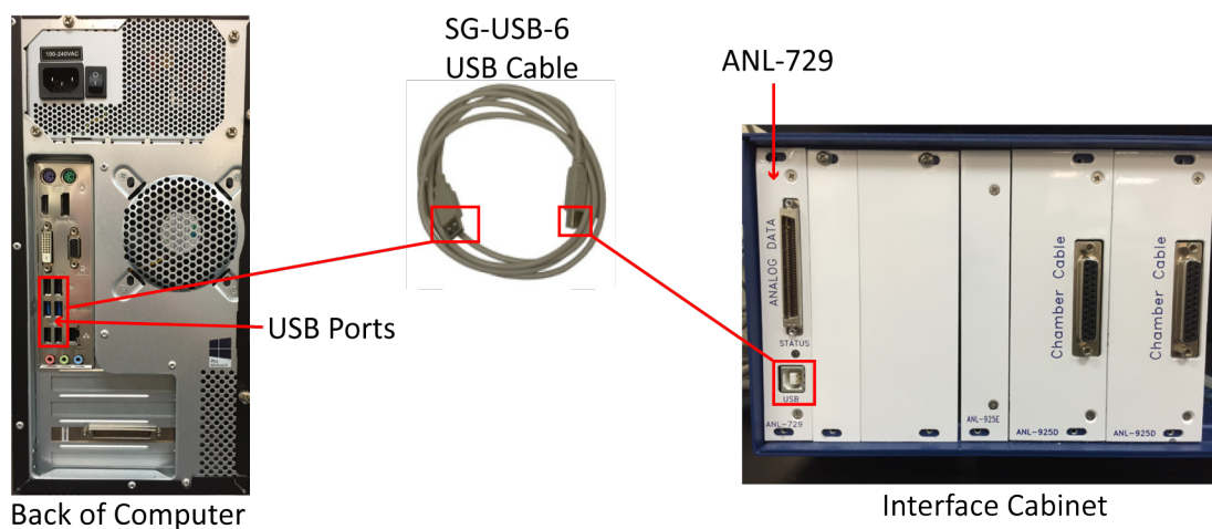
Figure 3-4 - Connect USB Port to ANL-729 Card
