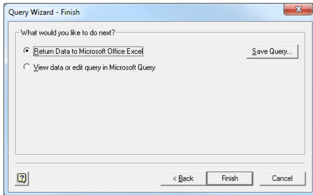
Figure 7-11 - Finish Screen
