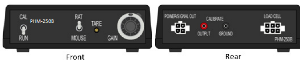
Figure 2-5 - PHM-250B Startle Load Cell Amplifier Front and Back Panel
