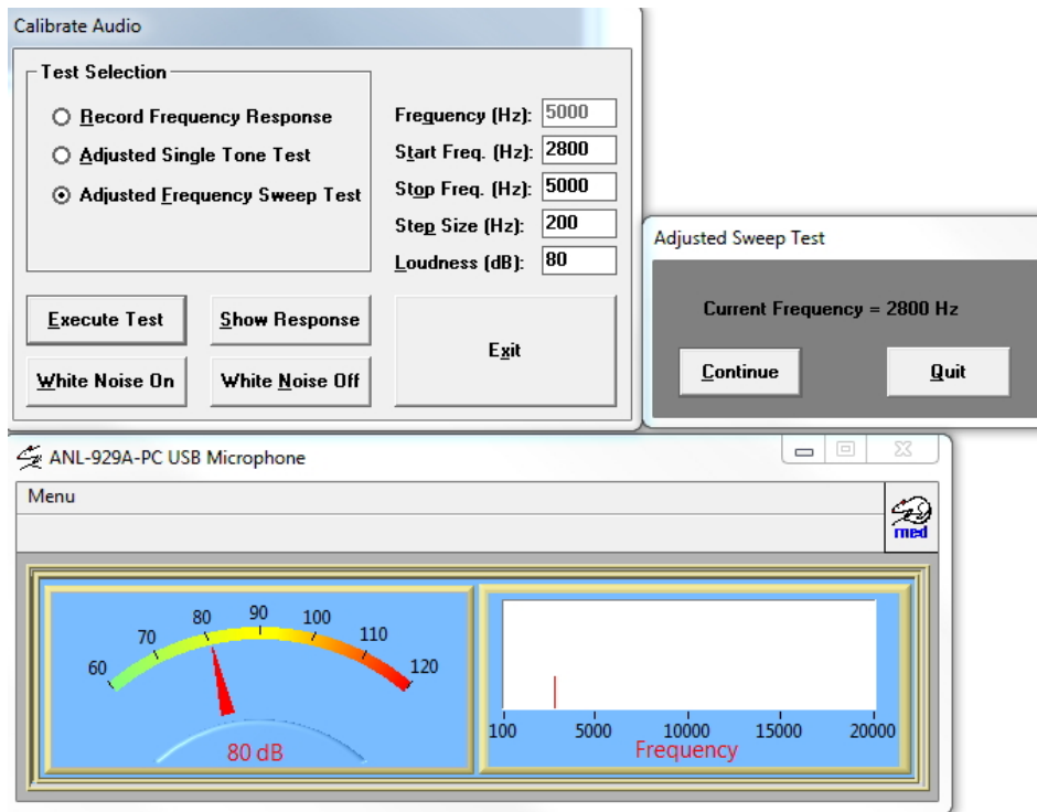
Figure 4-7 - Adjusted Frequency Sweep Test
