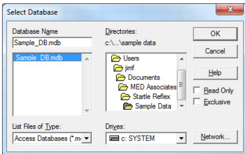
Figure 7-6 - Select Database
