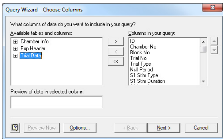
Figure 7-7 - Query Wizard
