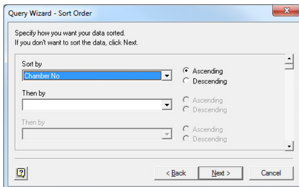
Figure 7-10 - Sort Order
