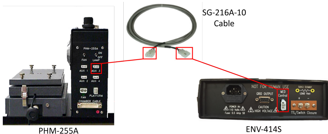
Figure 3-6 - PHM-255A Startle Platform to ENV-414S Aversive Stimulator
