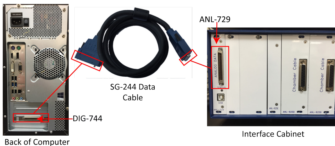
Figure 3-3 - Connect DIG-744 PCI Card to ANL-729 Card
