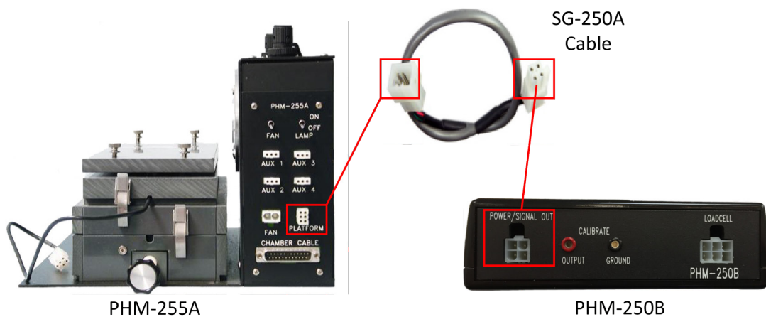
Figure 3-8 - PHM-255A Startle Platform to PHM-250B
