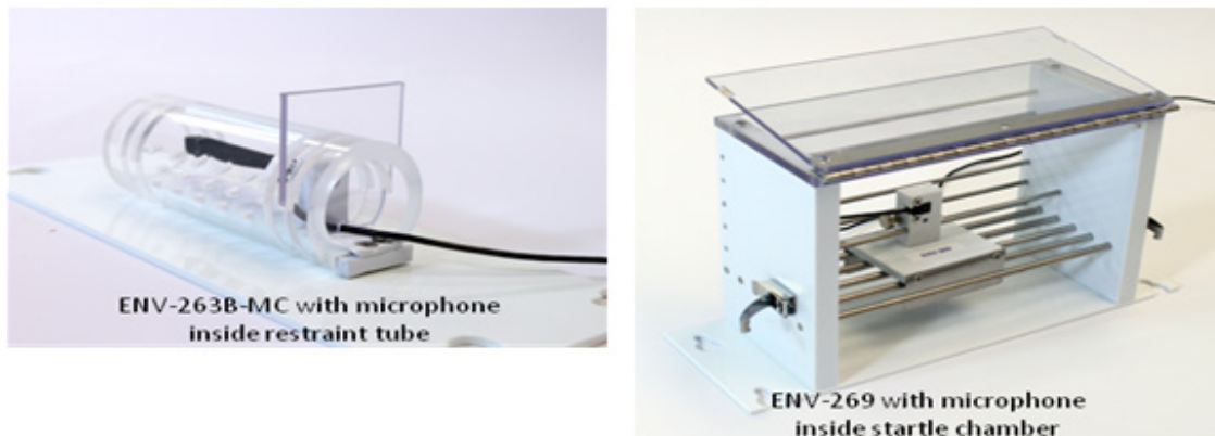
Figure 4-1 - Microphone calibrators
