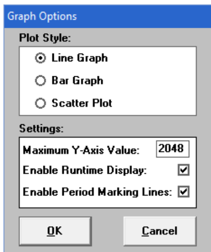
Figure 6-9 - Graph Options
