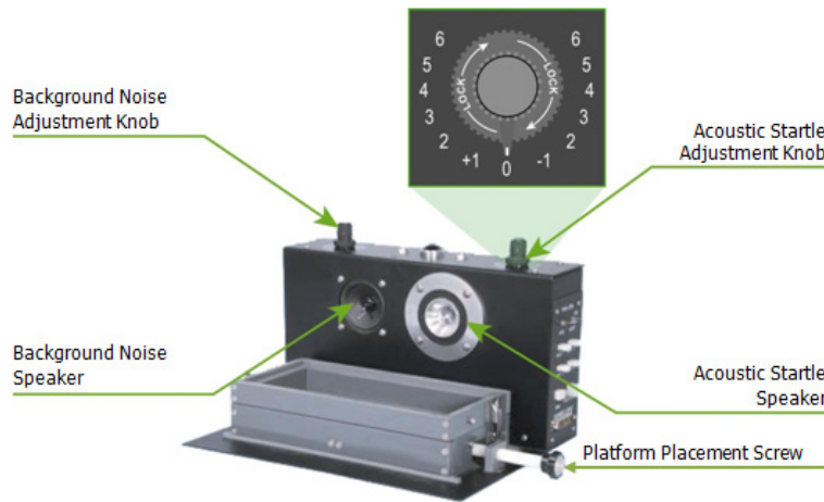
Figure 4-3 - PHM-255A Acoustic Startle Adjustment Knob
