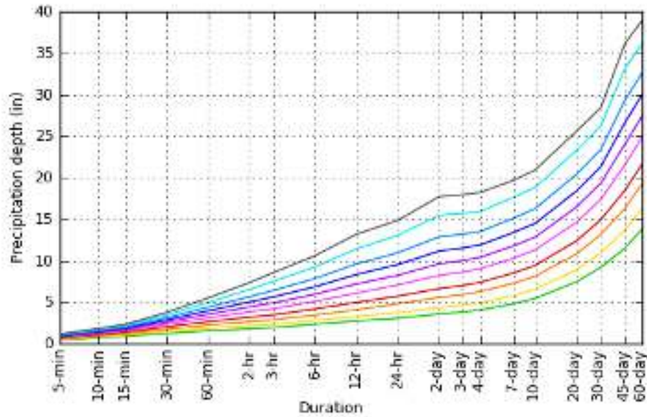
PDS-based depth-duration-frequency (DDF) curves Latitude: 36.5942°, Longitude: -76.4386°
