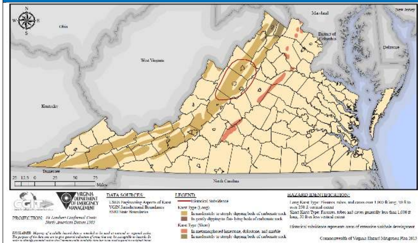
Figure 5.43: Karst Areas in the Commonwealth of Virginia
