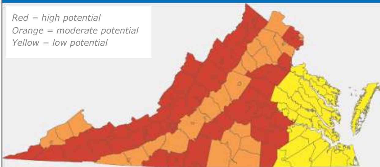
Figure 5.46: EPA Map of Radon Zones, Virginia
