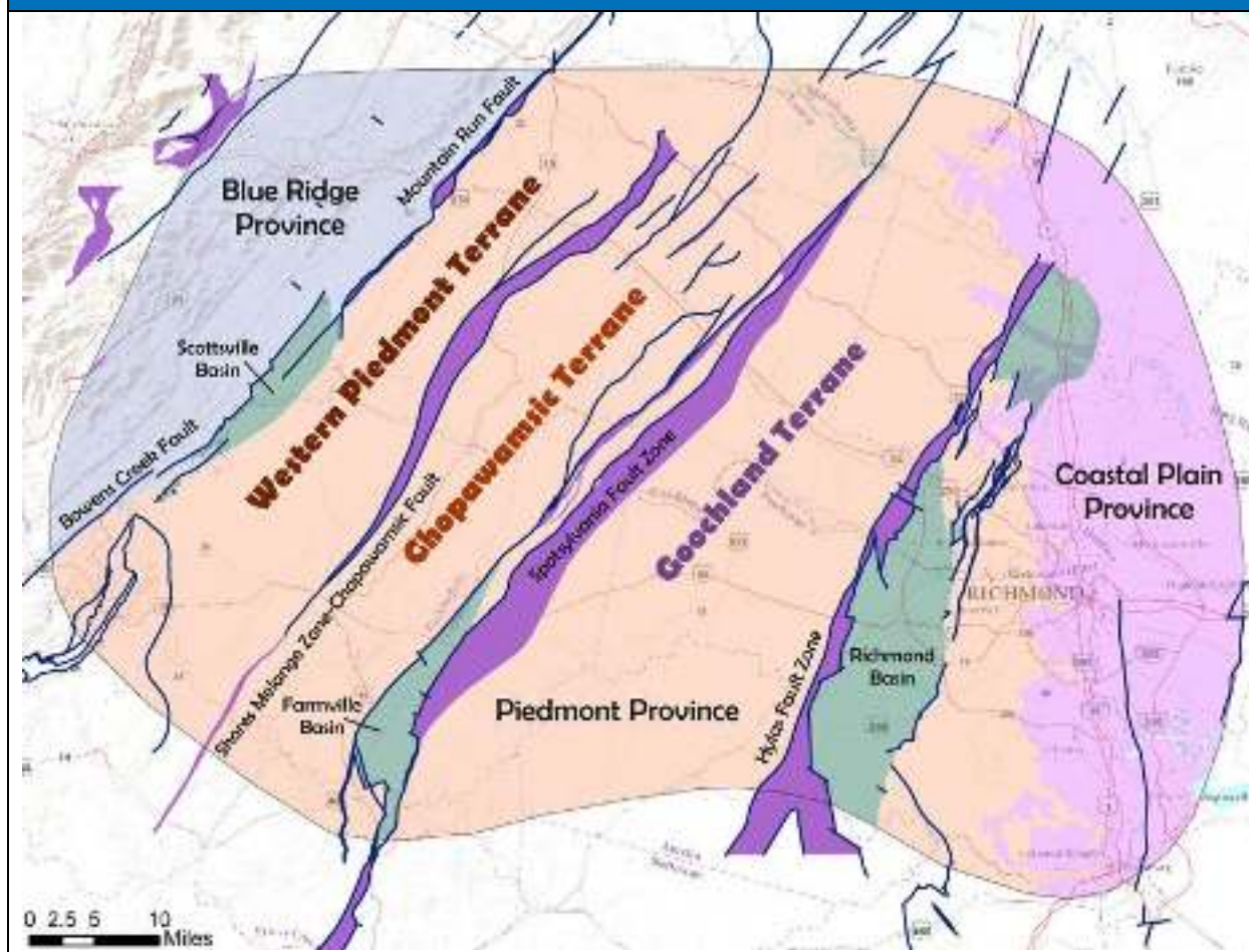
Figure 5.37: Major Faults and Tectonic Terranes within the Central Virginia Seismic Zone
