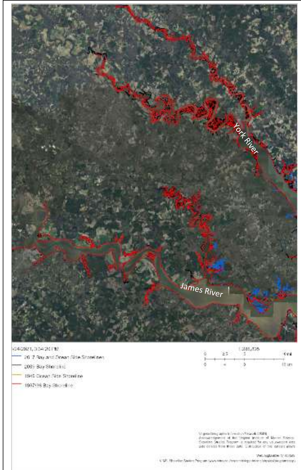
Figure 5.42: Regional Shoreline Change, 1937/38 - 2017
