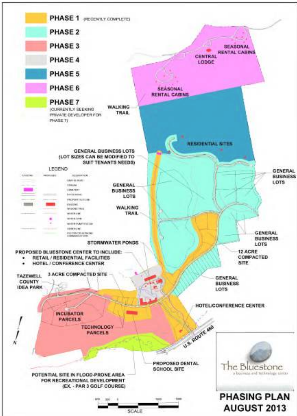
Figure 8.7 Site Plan Map of Bluestone
