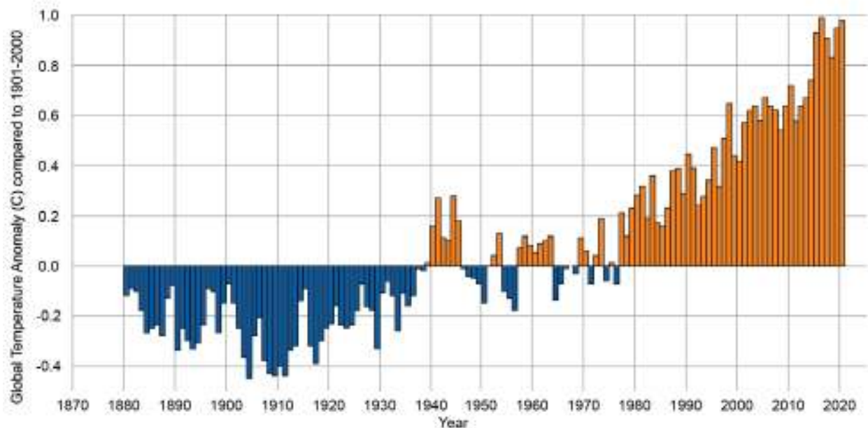
Figure 56: History of Global Ocean Surface Temperature Since 1880 194
