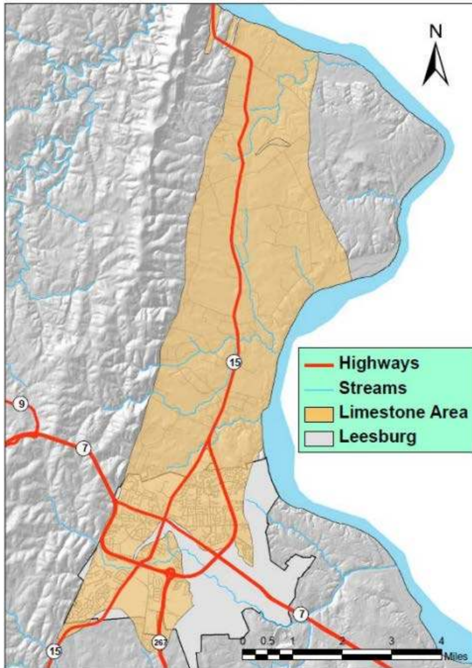
Figure 47: Loudoun County Limestone District 161
