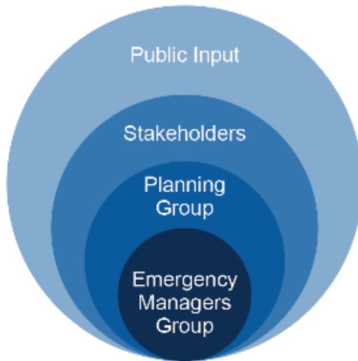
Figure 14: Planning Relationships
