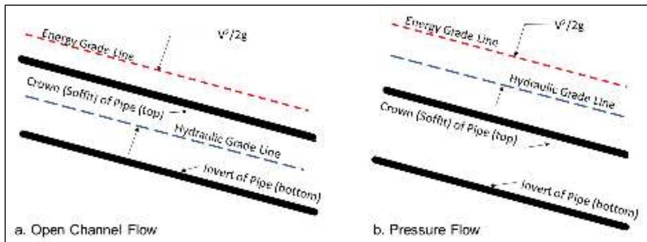
Figure 9.2. Hydraulic and energy grade lines in pipe flow.
