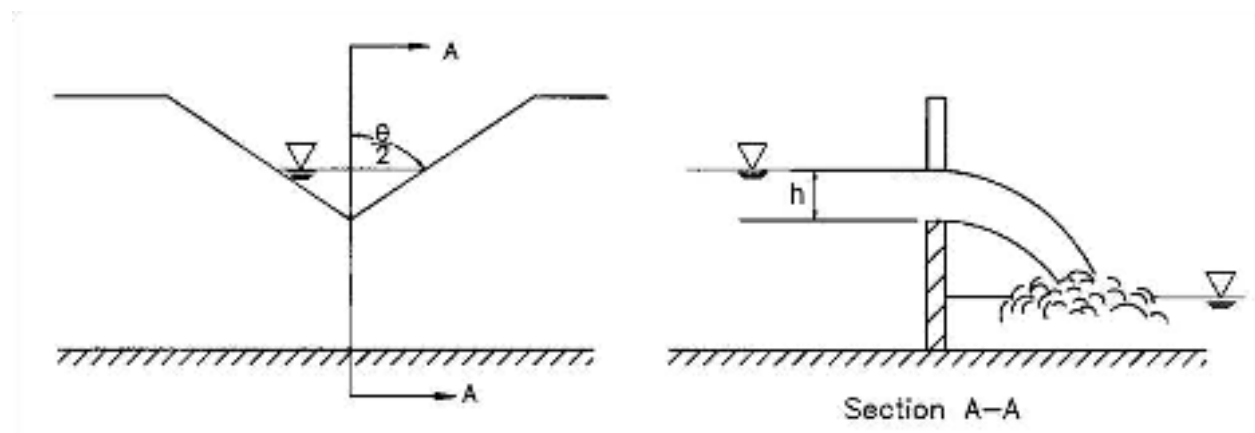
Figure 10.21. V-notch weir.
