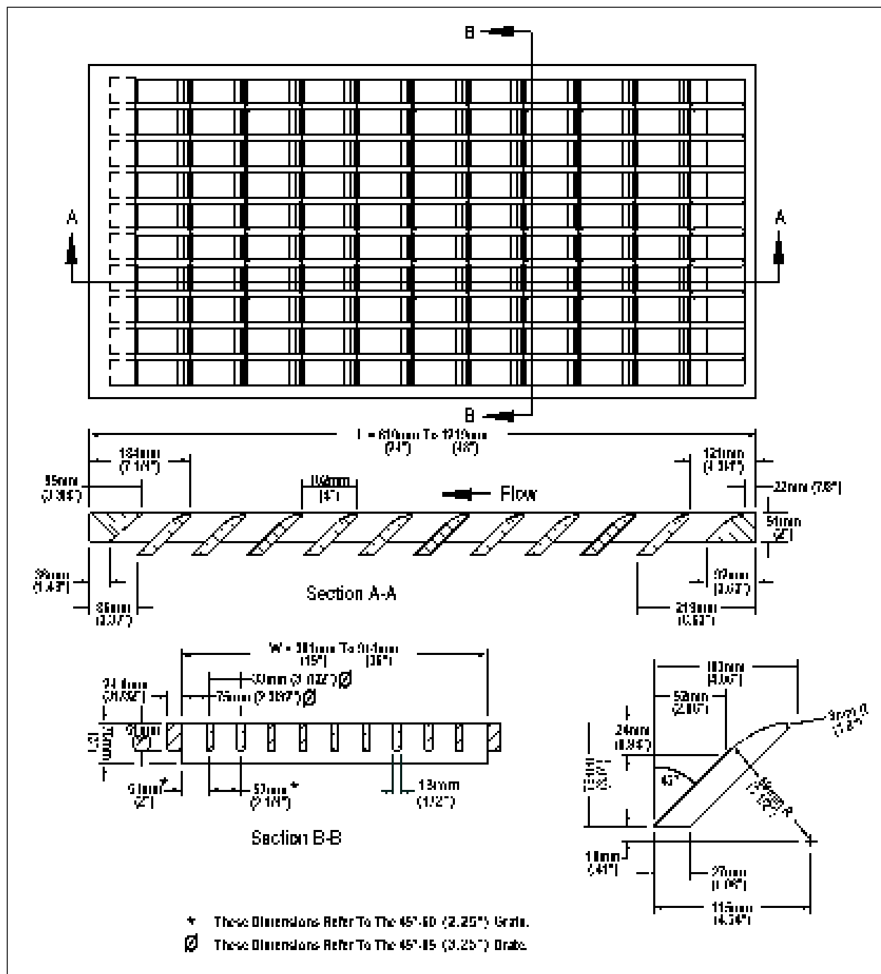
Figure 7.5. Tilt-bar grate: 45^\circ-60 (2.25 inch) and 45^\circ-85 (3.25 inch).
