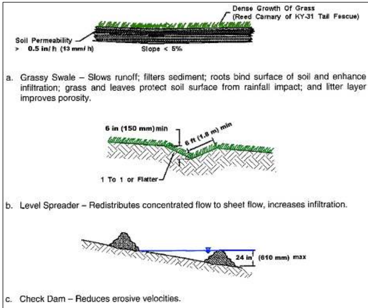
Figure 11.11. Schematic of grassed swale level spreader and check dam.
