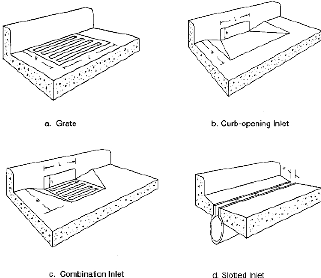
Figure 7.1. Storm drain inlet types.
