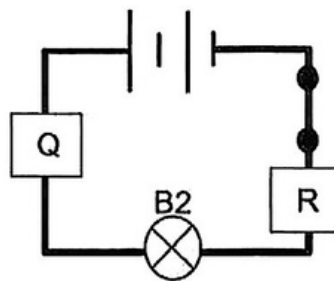
circuit 2
