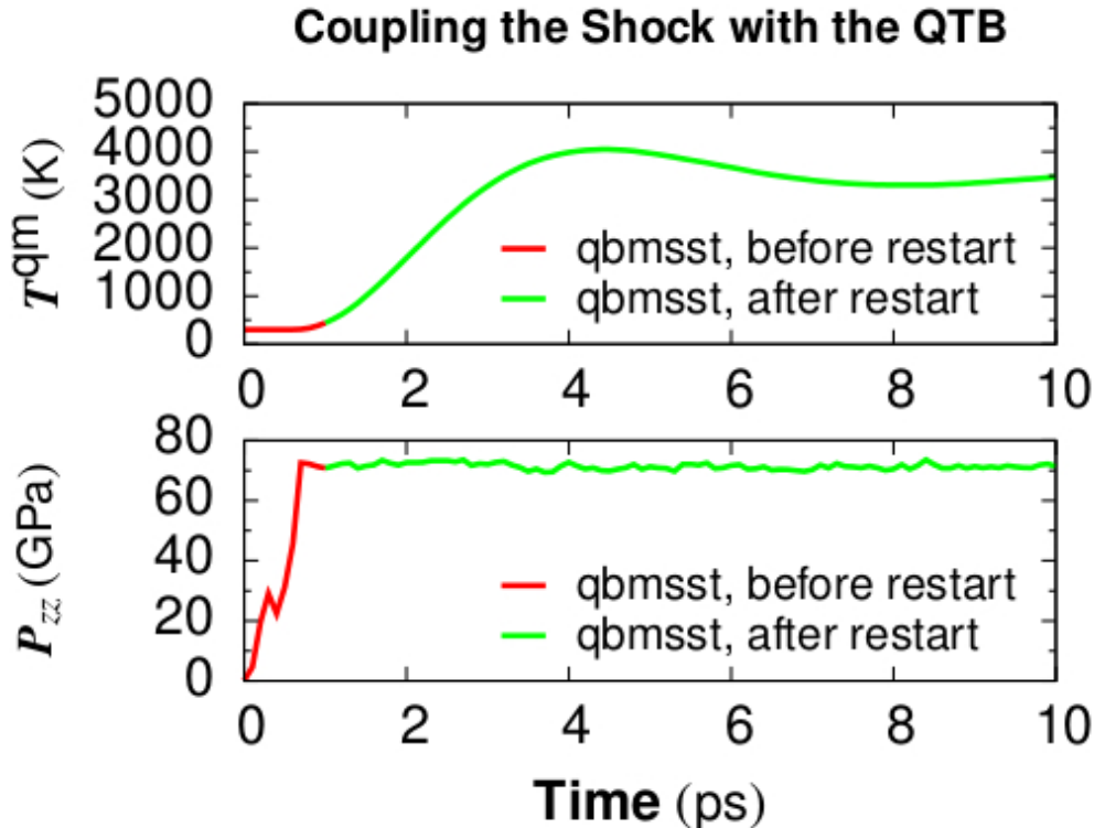
Figure 2. Quantum temperature and pressure vs. time for simulating shocked alpha quartz with the QBMSST. The shock propagates along the z direction. Restart of the QBMSST command is demonstrated in the example input script. Thermodynamic quantities stay continuous before and after the restart.
