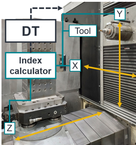
Fig. 3: Machine setup for adaptive condition mapping
