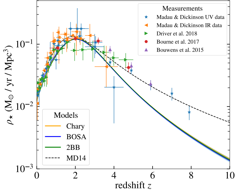
FIGURE 3.4.3: The SFRD as a function of redshift, with the 1\sigma uncertainty shown as light bands for each dust reemission model. Note that the bands overlap. Observational data compiled by Fermi-LAT Collaboration, Abdollahi, Ackermann, et al. (2018) are shown with different symbols. The parametrization of Madau and Dickinson (2014) (MD14 in the legend) is shown as a dashed line for comparison.
