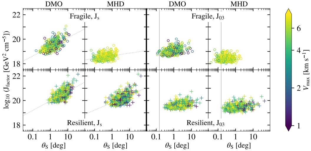
FIGURE 4.5.4: J-factor versus \theta_S for the brightest subhalo in 500 repopulations with V_{\max} \in [0.1, 8] km/s, with the colored z-axis representing the V_{\max} . We study different scenarios depending on subhalo resilience (fragile vs. resilient), definition of the J-factor used ( J_S and J_{03} , given by Eqs. (4.3) and (4.11), respectively), and inclusion of hydrodynamics (DMO vs. MHD). Vertical gray lines in the right J_{03} plots are placed at \theta = 0.15^\circ , i.e., the Fermi-LAT angular resolution at 1 GeV. Dotted gray lines on the left panels show log-log fits to the data.
