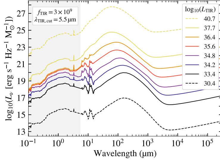
FIGURE 3.2.1: Set of synthetic spectra for dust reemission from ULIRGs (Chary and Elbaz, 2001). We use f_{\text{TIR}} = 3 \times 10^9 to convert between galactic and SSP luminosities, and \lambda_{\text{TIR,cut}} = 5.5 \mu\text{m} , represented by a shaded grey region below this value. We show the original spectra as solid lines, and our extrapolations as dashed lines.
