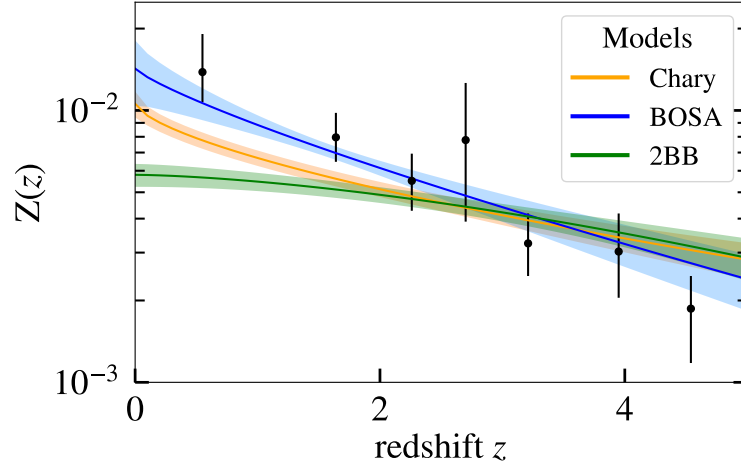
FIGURE 3.4.4: The mean metallicity Z as a function of redshift. Observational data is taken from Péroux and Howk (2020). The best-fit line and 1\sigma uncertainty are shown as a line and shaded region for each EBL model with a different dust reemission.
