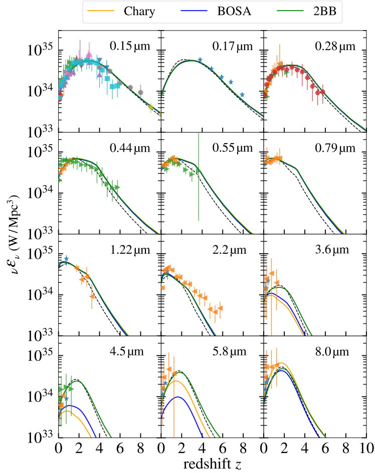
FIGURE 3.4.2: Emissivity data for specific wavelengths as a function of redshift. Observational data is taken from the compilation by Finke et al. (2022). Solid lines are our best-fit curves for each of our models. The 1\sigma uncertainty band is too thin to be seen. Model A from Finke et al. (2022) is shown as dashed black lines for comparison.
