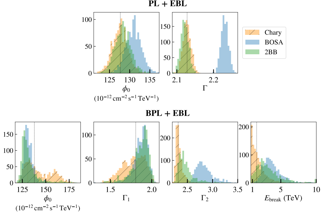
FIGURE 3.6.3: Best-fit parameters for the 1000 Poissonian pseudo-experiments assuming Chary is the true EBL model, for the fits performed with the three EBL models from Fig. 3.4.1. Dotted vertical lines are the best-fit parameters of the Asimov dataset. Parameters are given for the two spectral shapes studied in this work, listed in Table 3.6.1.
