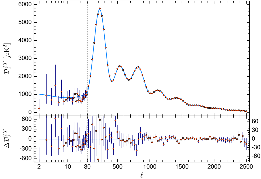
FIGURE 1.2: Planck 2018 temperature power spectrum as a function of the harmonic multipoles, shown as red markers. Best fit to the data as the blue curve. Vertical dashed line to separate two different parts of the data analysis in the original paper. At the bottom, residuals of the fit. Taken from Planck Collaboration, Aghanim, Akrami, et al. (2020).
