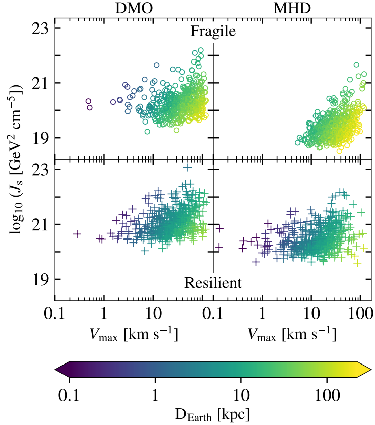
FIGURE 4.5.1: J_S (given by Eq. (4.3)) versus V_{\max} for the brightest subhalo in 500 repopulations with V_{\max} \in [0.1, 120] km/s, with the colored z-axis representing the distance to Earth. Different scenarios are shown depending on subhalo resilience (top and bottom panels for fragile and resilient populations, respectively) and inclusion or not of hydrodynamics (left for DMO; right for MHD).
