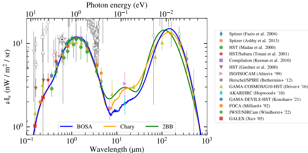
FIGURE 3.4.1: Overview of the EBL measurements used in this analysis. Data have been taken from Hill, Masui, and Scott (2018) and Biteau (2023). Upper limits of the EBL are represented as grey open symbols, lower limits as coloured filled symbols. More detailed description of the measurements is given in Section 3.3. The best-fit results of our EBL models with three different prescriptions for the dust reemission are also displayed, see Section 3.4.1.
