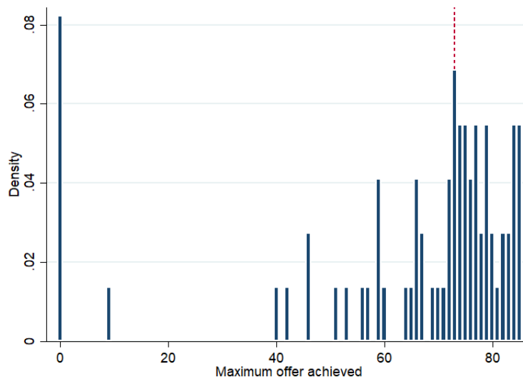
Figure 4: The histogram of maximum offers achieved in the high intensity treatment. The dashed red line represents the optimal threshold level of 73 in the alone search game.
