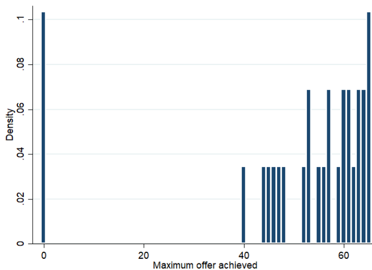
Figure 6: Histogram of maximum offers achieved in the outside option treatment
