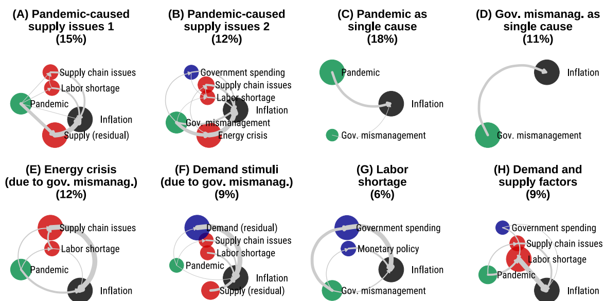
Figure E.3: Cluster analysis with Cosine distance
