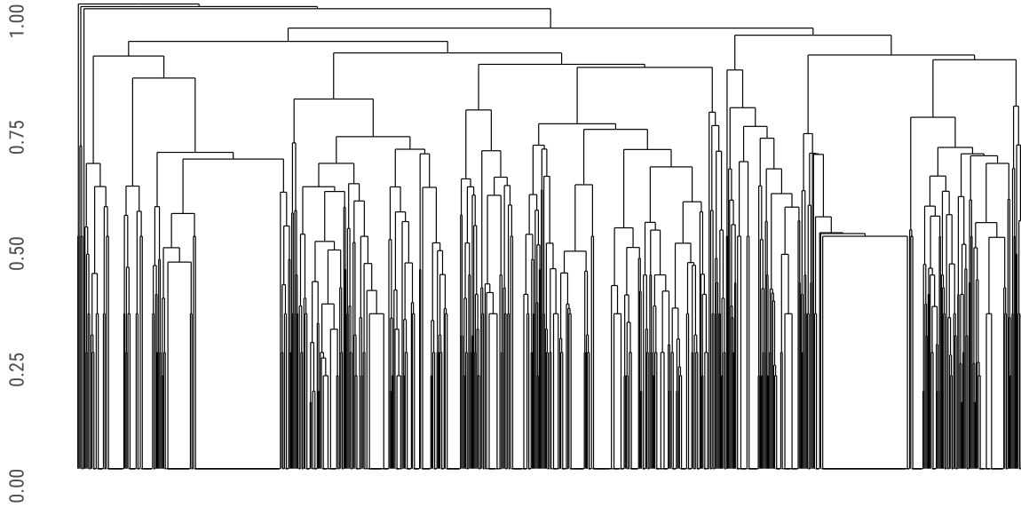
Figure E.1: Dendrogram
