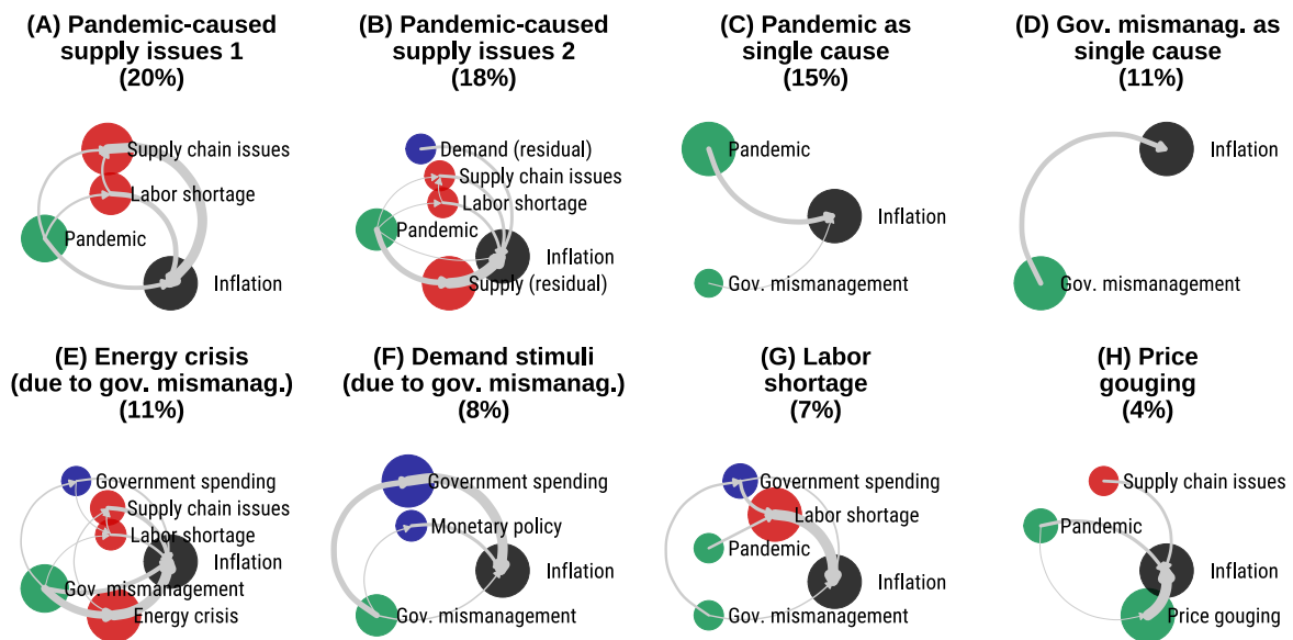
Figure E.2: Cluster analysis: main results (reproduced)
