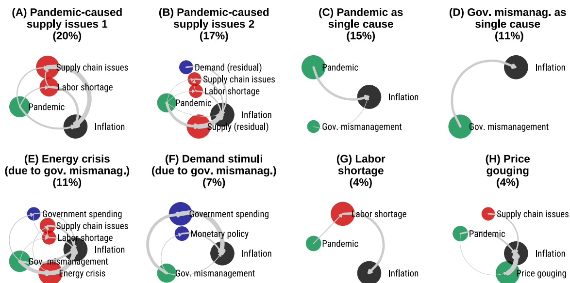
Figure E.4: Cluster analysis with 20 total clusters
