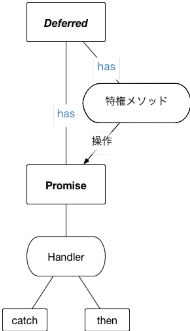
Figure 14. Deferred和Promise
