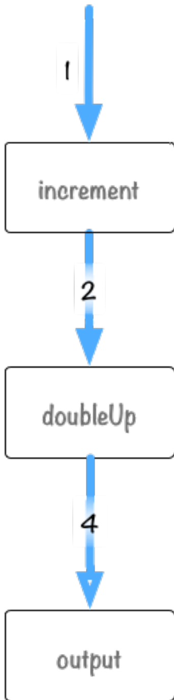
Figure 5. promise-then-passing-value.js 示意图
