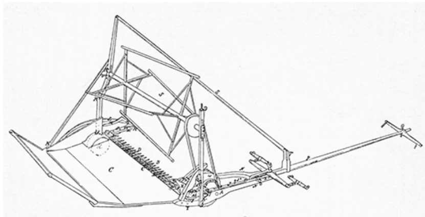
FIGURE 9.12 This sketch is from the 1845 patent for an improved grain reaper invented by Cyrus Hall McCormick. The reaper mechanized the labor-intensive use of scythes to harvest wheat.
