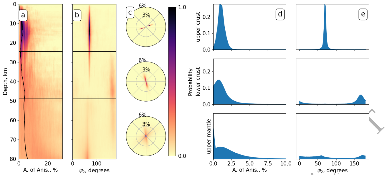
Figure 8. Depth inversion results for a sub-array located around 46.5^\circ N, 10^\circ E (location 4 of Figure 14). The solution is a large ensemble of models with different parameterizations (different number of isotropic and anisotropic layers). a) probability distribution of the amplitude of anisotropy (A. of Anis.). b) probability distribution of the direction of the fast axis of anisotropy. The black line in (a) shows the average amplitude and the horizontal black lines in (a) and (b) indicate the limits of the three layers over which we integrate anisotropy. c) Density plot of anisotropy parameters integrated over the 3 different depth ranges. The radius in the polar plots indicate amplitude and the angle gives direction of the fast axis of anisotropy. The colour scale indicates the normalised probability of a given combination of amplitude and fast direction. d) and e) show the marginal distributions of \delta V_s (d) and of \psi_2 (e) for each of the 3 depth ranges. The vertical scale is chosen such that the surface of the blue area is 1, i.e. the fraction of models with a given amplitude or ( \psi_2 ) range corresponds to the blue area within that range.
