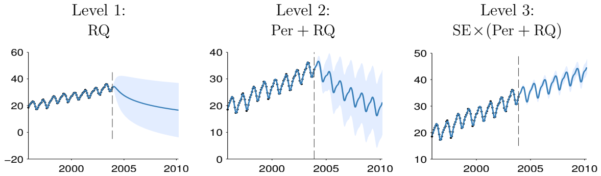
Figure 1.3: Posterior mean and variance for different depths of kernel search on the Mauna Loa dataset, described in section 1.6.1. The dashed line marks the end of the dataset. Left: First, the function is only modeled as a locally smooth function, and the extrapolation is poor. Middle: A periodic component is added, and the extrapolation improves. Right: At depth 3, the kernel can capture most of the relevant structure, and is able to extrapolate reasonably.
