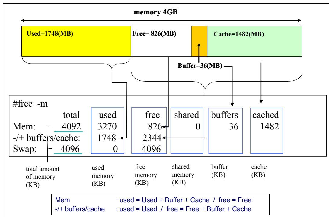
Figure 2-1 free command output
