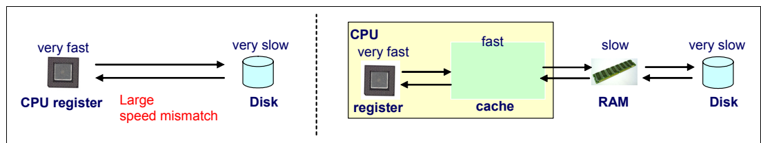
Figure 1-19 Memory hierarchy
