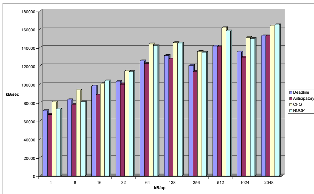
Figure 4-7 Random read performance per I/O elevator (synchronous)
