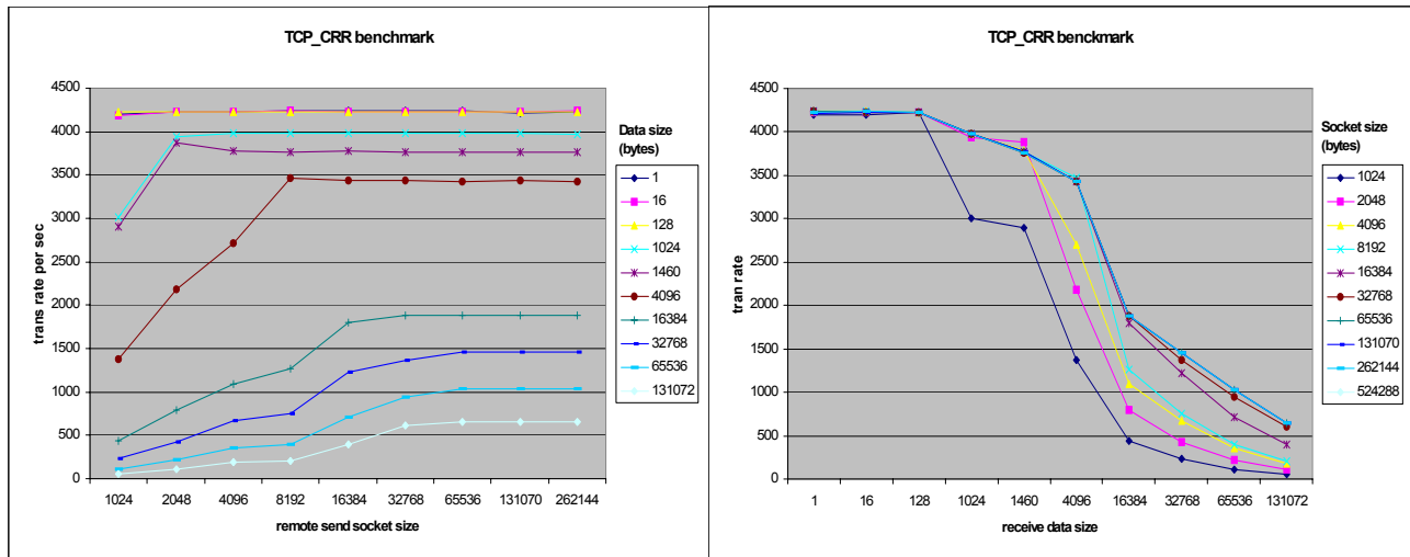
Figure 4-18 No Netfilter rule applied
