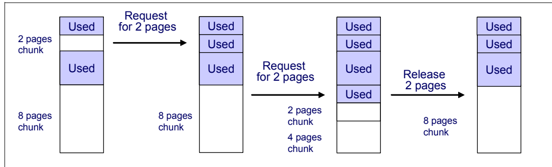
Figure 1-13 Buddy System
