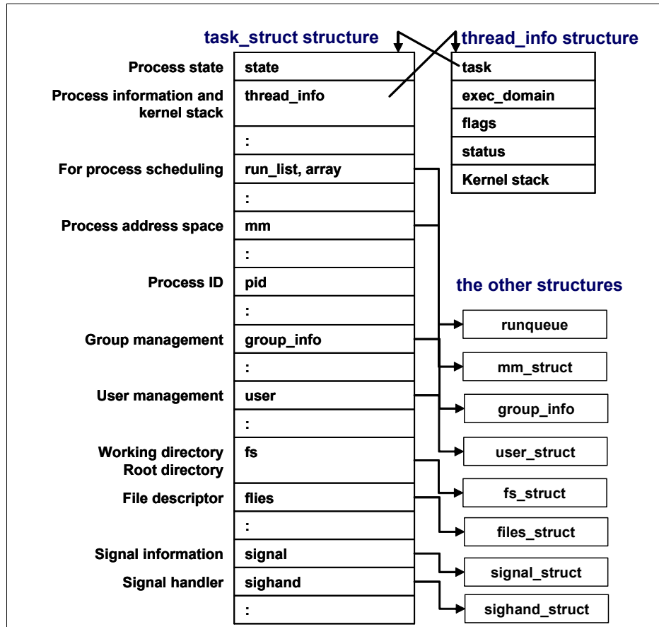
Figure 1-2 task_struct structure
