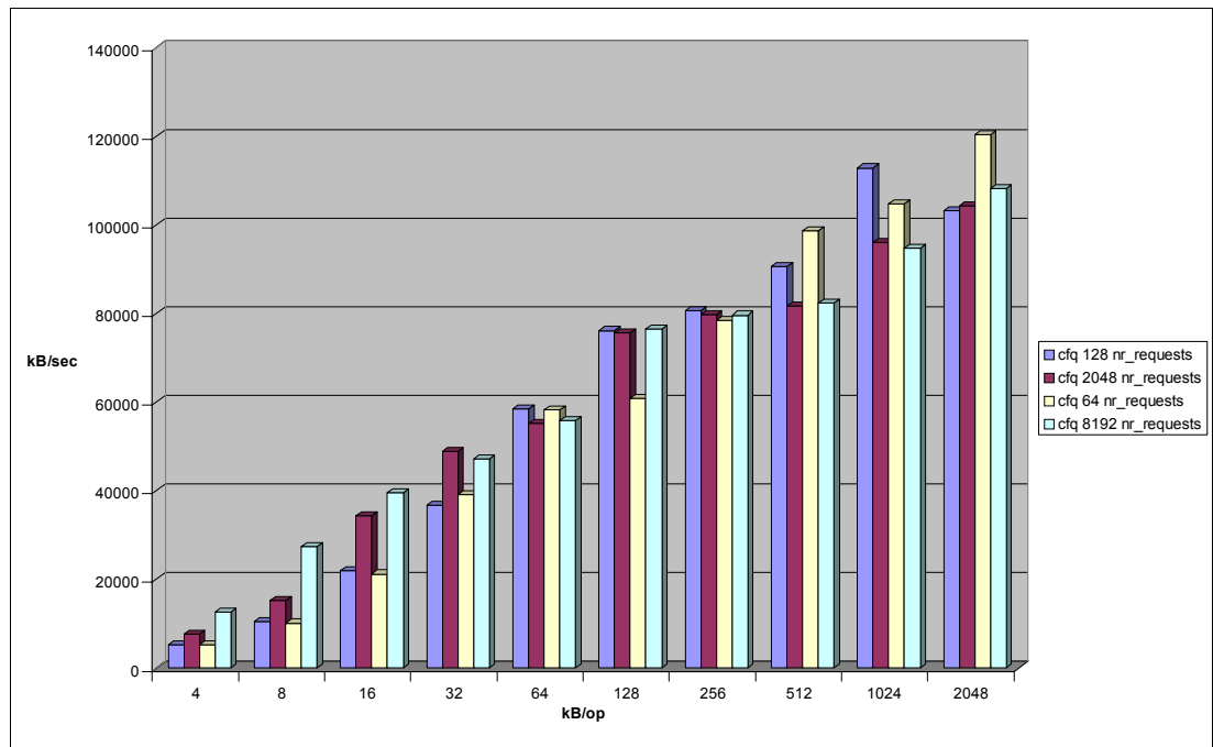
Figure 4-10 Impact of nr_requests on the CFQ elevator (random write Ext3)
