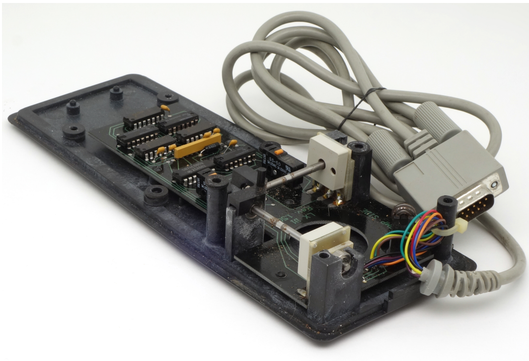
Figure 5: quadLYNX disassembled
