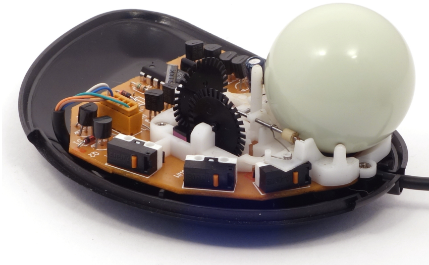
Figure 5: Colani Trackball disassembled
