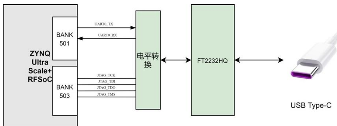
Figure 22: JTAG &amp; UART Connector Connection Diagram
