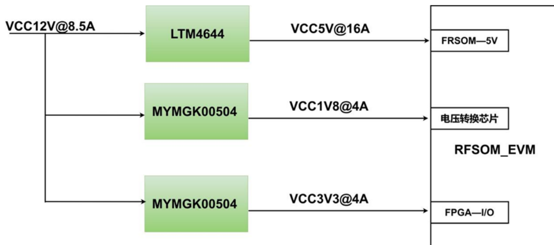
Figure 28: AXRF47 Carrier Board Power Interface Section
