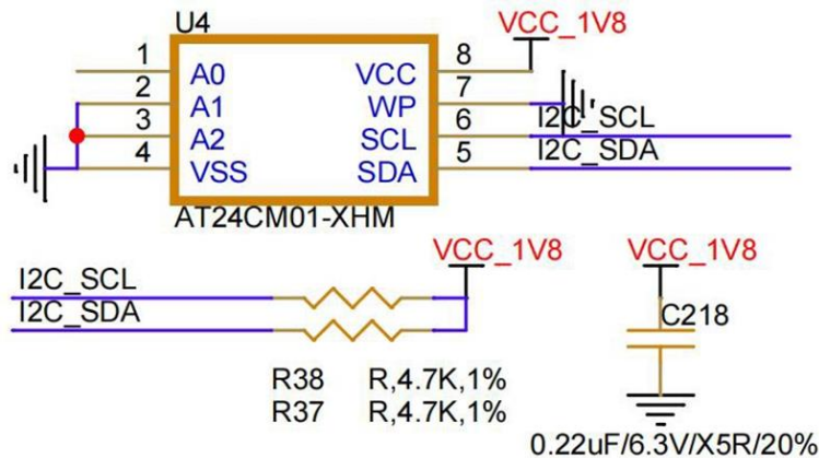
Figure 8: EEPROM Hardware Schematic
