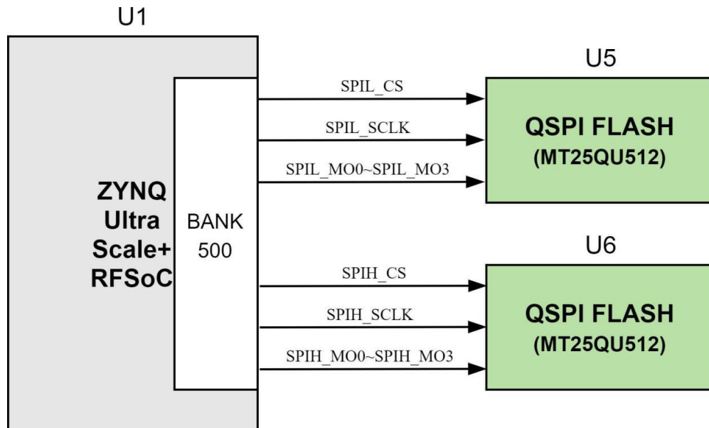
Figure 7: QSPI FLASH Connection Diagram
