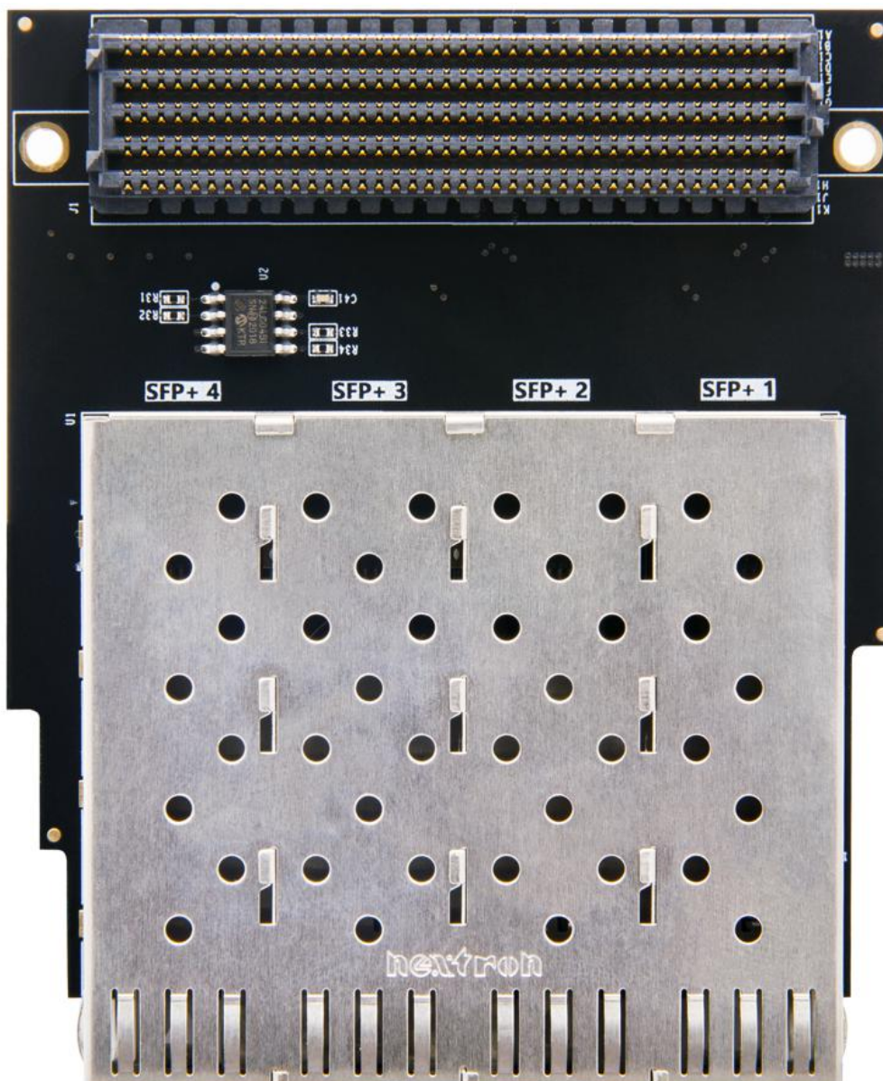
Figure 1-1: FH1223 Module
