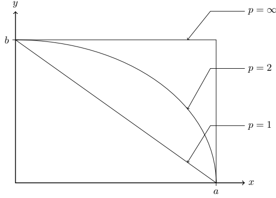
Figure 1: Boundaries of B_{S_p}(a, b)|_{\mathbb{I}^2} for different p .
