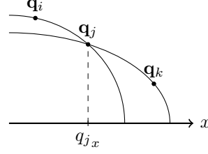
Figure 2: Illustration of Lemma 3.
