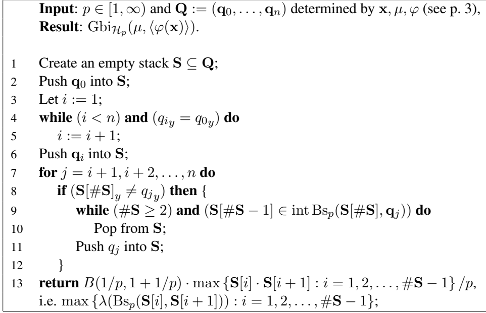
Figure 3: Algorithm for computing \text{Gbi}_{\mathcal{H}_p}(\mu, \langle \varphi(\mathbf{x}) \rangle) , for 1 \leq p < \infty .
