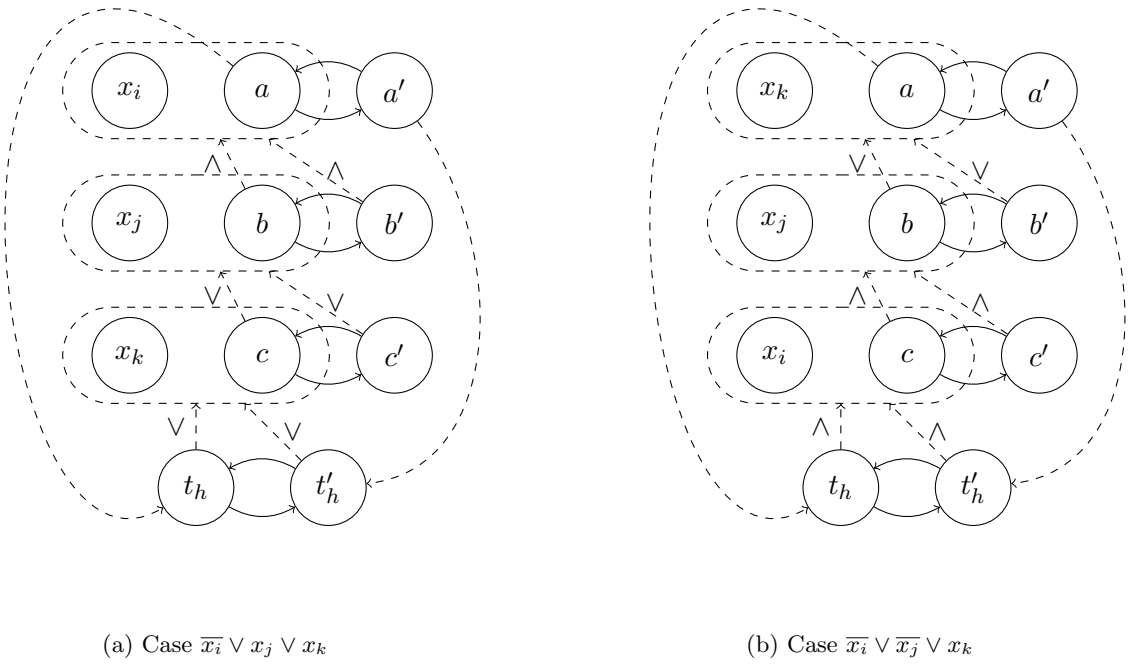
Figure 4: Gadgets for MINMAX
