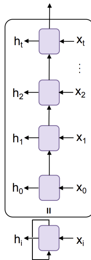
(a) RNN
