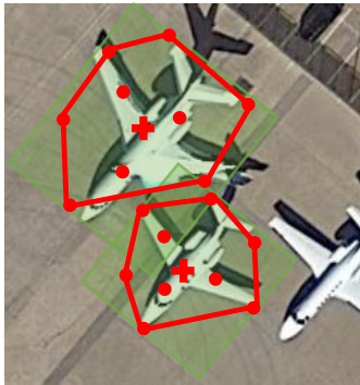
Convex-hull Generation
