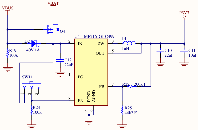
DC-DC CONVERTOR
