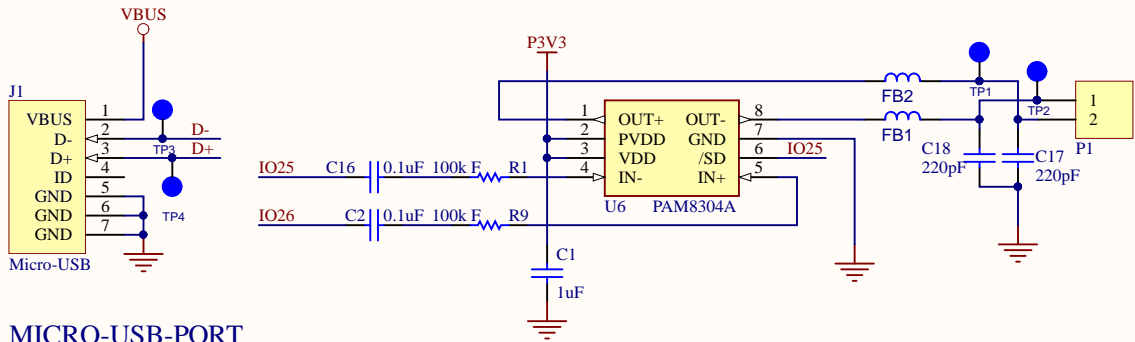
MICRO-USB-PORT
