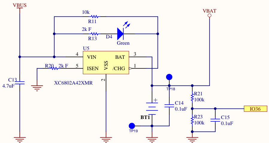
BATTERY CHARGER
