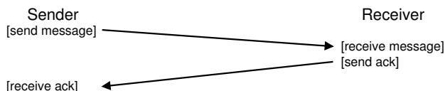
Figure 48.3: Message Plus Acknowledgment
